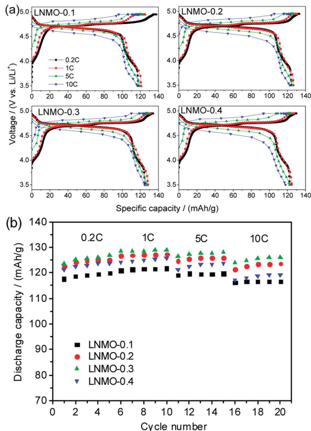
Fig. 4 Charge/discharge curves at various rates (a) and rate capability curves (b) for LiNi 0.5 Mn 1.5 O 4 samples synthesized at different reactant concentrations.
