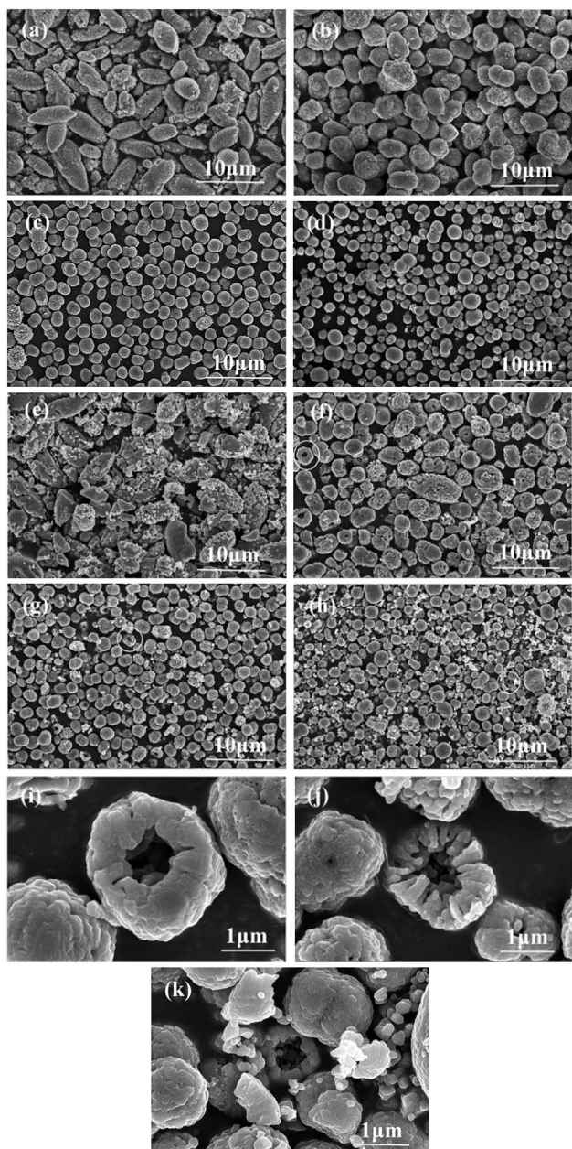
Fig. 3 SEM images of carbonate precursor (a–d) and LiNi 0.5 Mn 1.5 O 4 samples (e–k) (a and e) 0.1 mol L -1 , (b, f and i) 0.2 mol L -1 , (c, g and j) 0.3 mol L -1 , (d, h and k) 0.4 mol L -1 .
