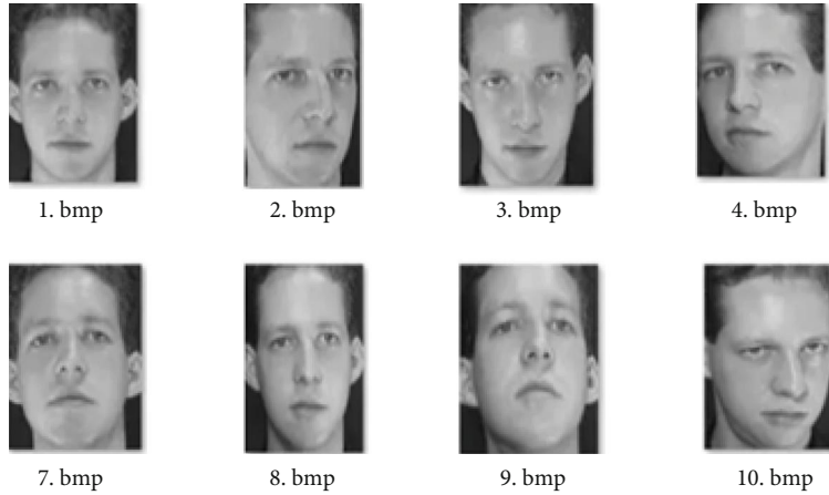
FIGURE 12: ORL dataset.
