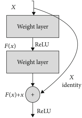
FIGURE 7: Structure diagram of shortcut connect.
