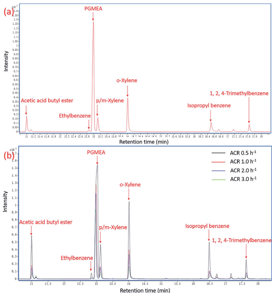
Fig. 3 Chromatograms of VOCs emissions at 24 h from the medium density fibreboard coated with oil-based paint: (a) at ACR 1.0 h -1 ; (b) at different ACR conditions.
