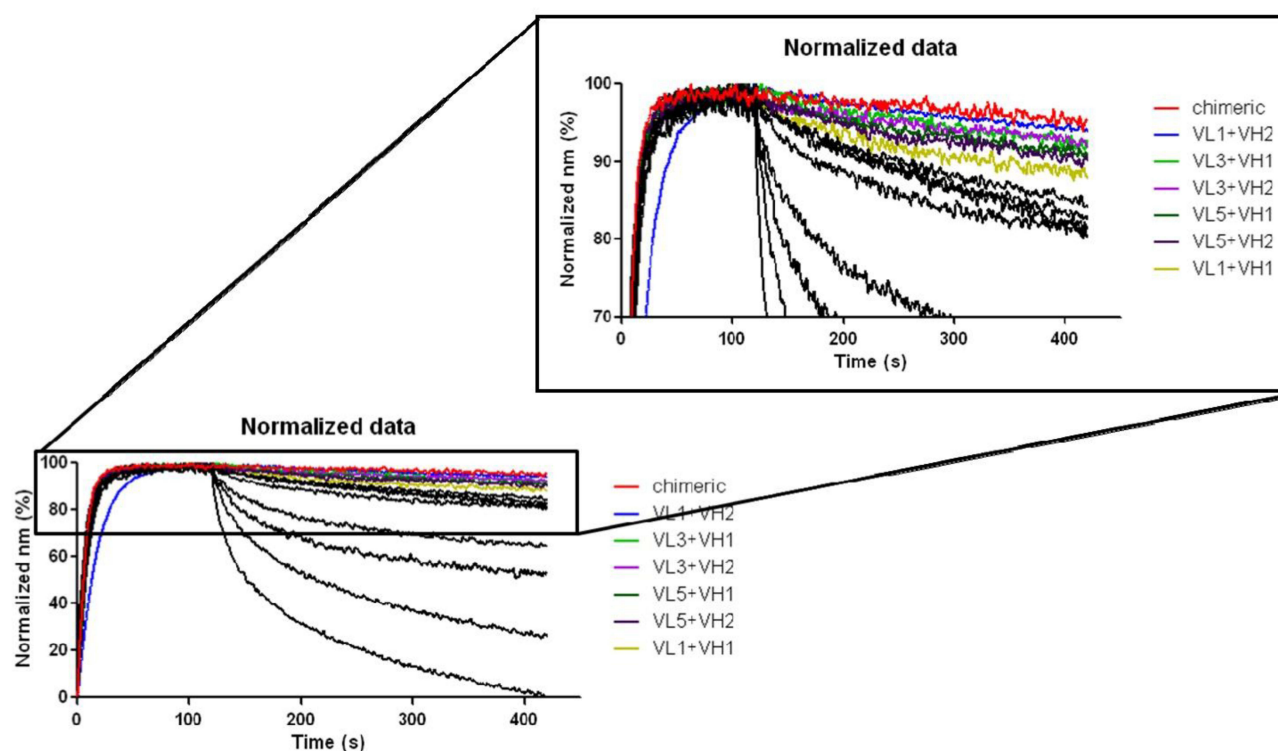
Figure 2 Binding behavior analysis and affinity ranking of humanized antibodies on AHC sensor using OctetRed96. Humanized antibody variants were ranked based on their off-rates using OctetRed 96. The assay was performed at 30°C in 1×Kinetics assay buffer (1×PBS, 0.05% Tween-20, pH 7.4). Agitated samples were captured by humidified AHC sensors. The association was allowed for 120 seconds. One concentration (100 nM) of analyte (ie antigen protein) was used. The dissociation was monitored for 300 seconds. In order to compare the off rates of chimeric and humanized variants, the experimental raw data were normalized at the beginning of the dissociation.
