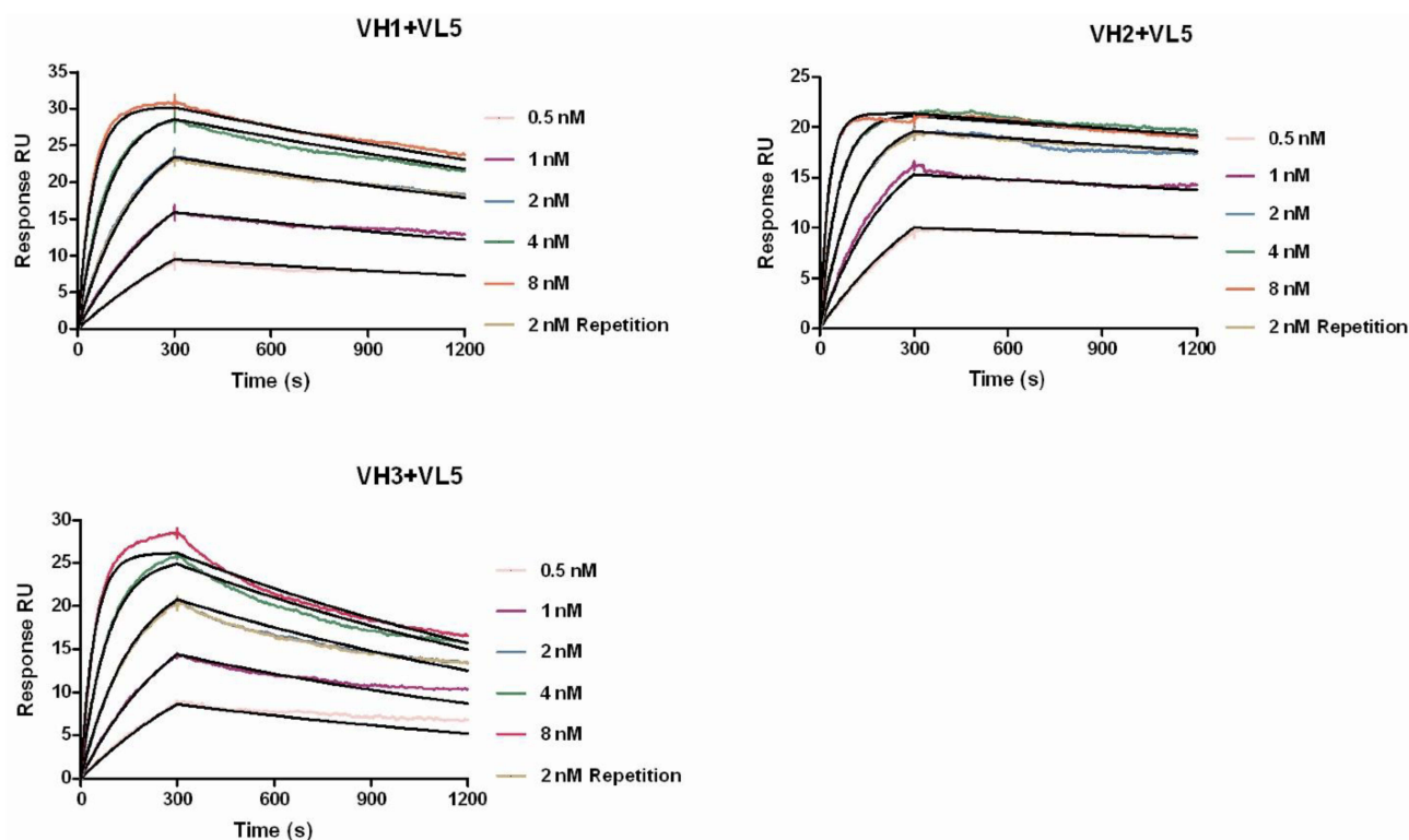
Figure 3 Antibody-antigen affinity measurement using Biacore T200. Affinity measurement using Biacore T200 was carried out following GE's handbook. A binding analysis cycle consists of three steps: (i) capture of the ligand (ie humanized IgG) onto the sensor chip surface by the immobilized anti-Human antibody; (ii) binding of the analyte (ie antigen protein, increasing concentration ranging from 0.5 nM to 8 nM) to the ligand; (iii) dissociation of bound analyte. Sensor surface was regenerated after each binding cycle using the manufacturer's recommended conditions. All binding cycles were run at 25°C. The binding affinities of variants VH1+VL5, VH2+VL5 and VH3+VL5 are shown. Black curves represent the fit of Langmuir 1:1 interaction model to experimental data. The antigen concentrations are 0.5 nM, 1 nM, 2 nM, 4 nM and 8 nM; experiment at antigen concentration of 2 nM was repeated for reference.
