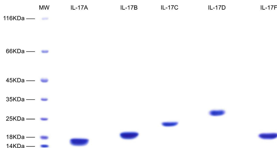
Figure 1 Purity analysis of IL17 isoforms by Electrophoresis (4–20% gradient SDS-PAGE). 10µL of each purified IL-17 isoform was loaded on to the 4–20% gradient SDS-PAGE. As shown in the PAGE analysis, all the five proteins are reasonably pure enough to carry out ELISA and other assays.
