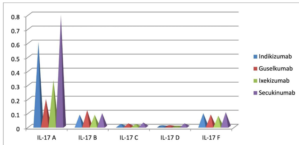
Figure 6 Determination of Binding specificity of anti-IL17 antibodies to IL17 isoforms. 200 ng of recombinant E. coli expressed IL-17A, B, C, D, F were coated in the plate and above listed Goat anti-Human IgG-Fc-HRP was employed as the secondary antibody at a dilution of 1:5000, primary antibodies used at 100 ng/well. Except Guselkumab all other antibodies are showing some degree of binding affinity to IL-17A antigen. All the antibodies show no binding affinity towards IL-17B, C, and D. Very little or no binding affinity is observed against IL-17F. Indikizumab; humanized antibody against IL17A, Ixekizumab; humanized antibody against IL-17A/F, Guselkumab; completely human monoclonal antibody that binds to the interleukin (IL)-23 p19 subunit specifically and prevents it from interacting with the IL-23 receptor; Secukinumab is a human IgG1 \kappa monoclonal antibody neutralizes IL-17A.
