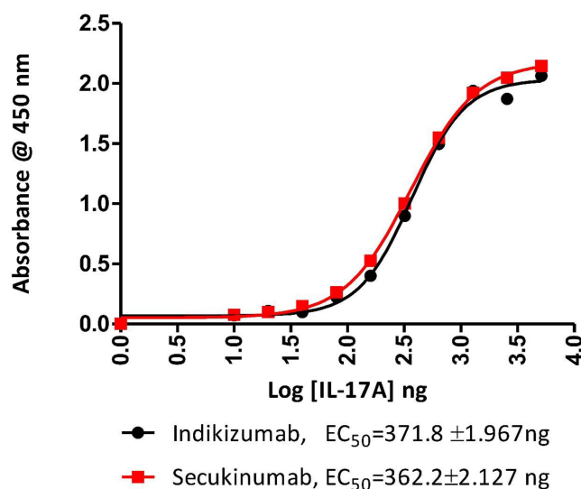
Figure 7 Comparative In vitro efficacy study between Indikizumab and Secukinumab by ELISA. Different concentration of recombinant- IL-17A (10ng-5120ng/well) were coated in the 96 well ELISA plate and incubated overnight at 4°C. Indikizumab and (Secukinumab) produced in CHO-K1 were used as the primary antibody at concentration of 100 ng/well. After the washing procedure binding signal was amplified and detected using Goat-Anti-Human IgG-Fc (1:5000 dilution). TMB Substrate used at 1x from 5x Stock. Statistical analysis was done using Log [Antigen] vs response- variable slope.
