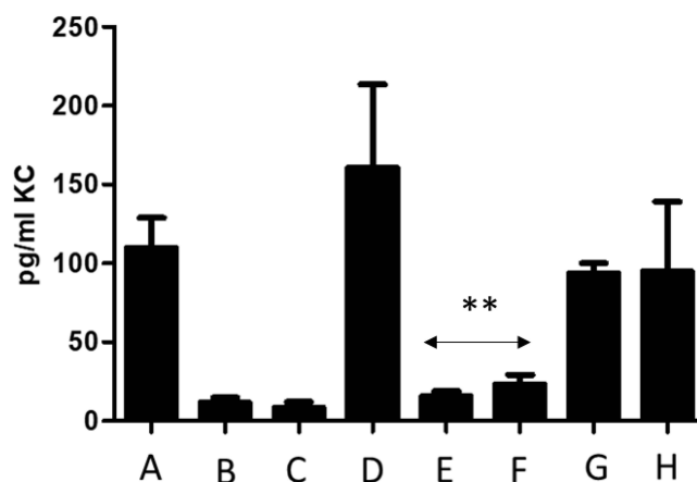
Figure 9 Indikizumab inhibits Human IL17A induced KC (Keratinocyte) secretion in C57BL/6 mice. C57BL/6 mice were given subcutaneous injections of human IL-17A (3 µg) one hour after receiving an IV injection of indikizumab (1 mg/kg, 0.1 mg/kg, 0.01 mg/kg, or 0.001 mg/kg) (ie, 20 µg, 2 µg, 0.2 µg, and 0.02 µg per mouse, respectively). Using ELISA, KC levels were determined 2 hours post human IL-17A injection. n=3 mice per group. Indikizumab treatment accounts for 68.99% of total variance. P value=0.0065** (If Indikizumab Treatment has no effect overall, there is a 0.65% chance of randomly observing an this big (or bigger) in an experiment of this size. The effect is considered very significant.). Group A-Human IL-17A 3 µg/mouse, B-Indikizumab 20 µg/mouse, C-Human IgG1 Isotype control 20 µg/mouse, D-Human IL-17A +Isotype control IgG1 20 µg/mouse, E- Human IL-17A+Indikizumab 20 µg/mouse, F- Human IL-17A+Indikizumab 2 µg/mouse, G- Human IL-17A+Indikizumab 0.2 µg/mouse, H- Human IL-17A+Indikizumab 0.02 µg/mouse.
