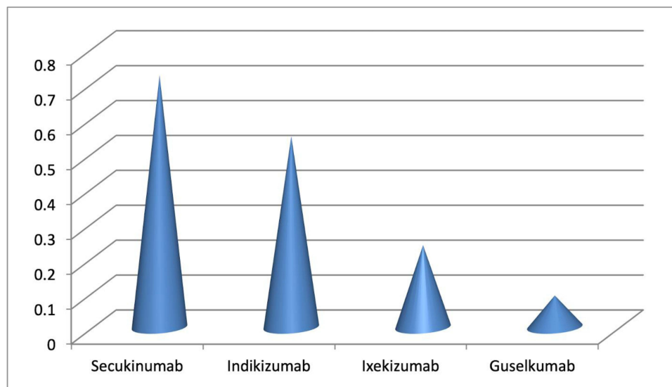
Figure 5 Comparative Immuno-affinity assessment of antigen-antibody by Enzyme Linked Immunosorbent Assay. 200 ng of E. coli expressed recombinant IL-17A was coated in the plate and above listed goat anti-human IgG-Fc-HRP was employed as the secondary antibody at a dilution of 1:5000, whilst antibodies (100 ng/well) were utilized as the primary antibody. Secukinumab and Ixekizumab are showing variable degree of affinity whereas, Guselkumab does not show any binding suggesting its specificity towards IL-23, at the same time our in-house developed Indikizumab shows binding affinity at par with Novartis Secukinumab. Indikizumab; humanized antibody against IL17A, Ixekizumab; humanized antibody against IL-17 A/F, Guselkumab; human monoclonal antibody that binds to the interleukin (IL)-23 p19 subunit specifically and prevents it from interacting with the IL-23 receptor; Secukinumab is a human IgG1 \kappa monoclonal antibody neutralizes IL-17A.
