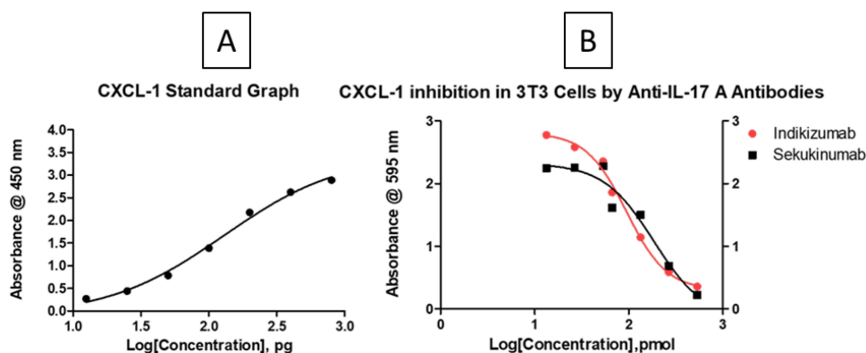
Figure 8 Comparative analysis of CXCL-1 inhibition in NIH 3T3 cells by Indikizumab and Secukinumab. (A). CXCL-1 Standard Graph; CXCL-1 (0–800 pg/well). (B). 3T3 cells were treated with pre-incubated mixture of Recombinant- IL-17A (60 ng/well) with Indikizumab & Secukinumab (13–533 pmol/well) for >60 hours. Culture supernatant was harvested and tested in ELISA. CXCL-1 capture antibody was coated in the 96 well ELISA plate and kept overnight. Following the SOP of blocking, binding and washing, detection antibody at concentration 100 ng/well was added. After the washing procedure binding signal was amplified and detected using Avidin-HRP (1:1000 dilution). TMB Substrate used at 1x from 5x Stock. Statistical analysis was done using Non-linear regression of Log (Concentration) vs response. At 95% Confidence Intervals; Log [IC 50 ] = Indikizumab = 1.976 ± 0.058; Secukinumab = 2.26 ± 0.28 pmol.
