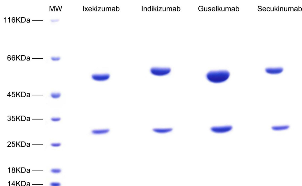
Figure 4 Purity analysis of anti-IL17 antibodies produced in transiently transfected CHO-K1 cell line by Electrophoresis (4–20% gradient SDS-PAGE). 10 \mu L of affinity (MabSure Select, Cytiva) purified antibodies were treated in the SDS-PAGE sample buffer for reduction. Boiled samples were loaded on to the gel for electrophoresis. All the four antibodies are relatively pure and the light chain and heavy chains migrated at the desired molecular weight in SDS-PAGE.
