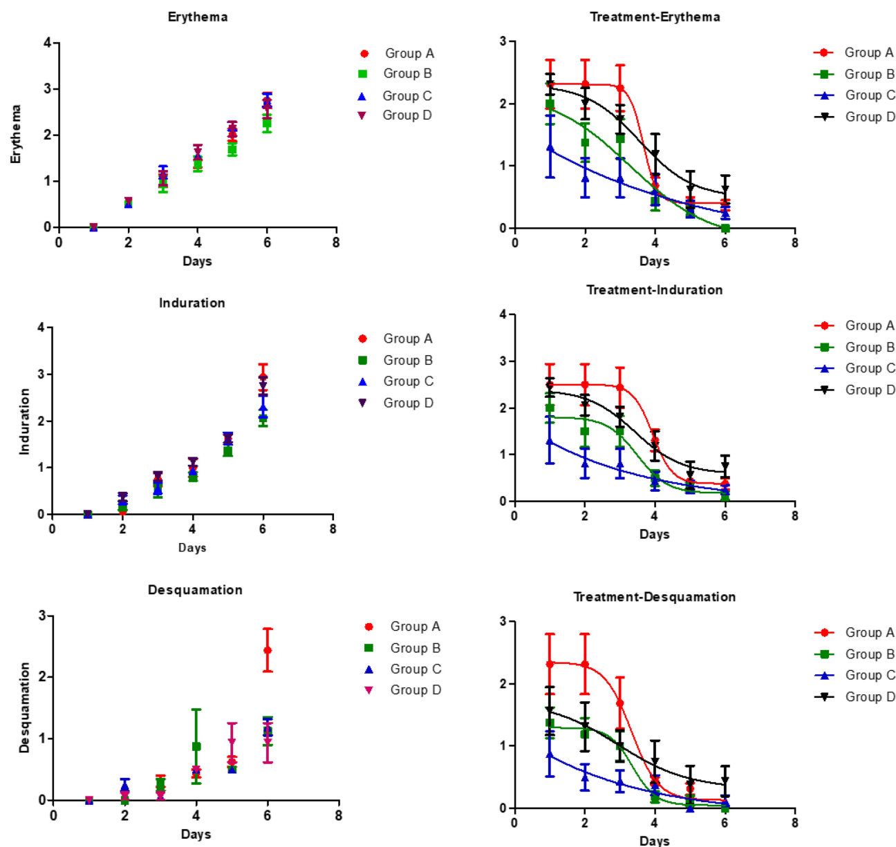
Figure 10 Indikizumab and Secukinumab Inhibit IMIQUIMOD induced psoriasis in mice. Eight to 11 weeks old BALB/c mice received a daily topical dose of 62.5 mg of commercially available IMQ cream (5%) (IMIQUIMOD, from Glenmark) on the shaved back for 6 consecutive days, translating in a daily dose of 3.125 mg of the active compound. Control mice were treated similarly with Vaseline. The animals were treated with 48 \mu g/mouse/day single dose of antibody. Group A- Control; Group B- Mouse Anti-IL-17A; Group C-Indikizumab; Group D- Secukinumab.
