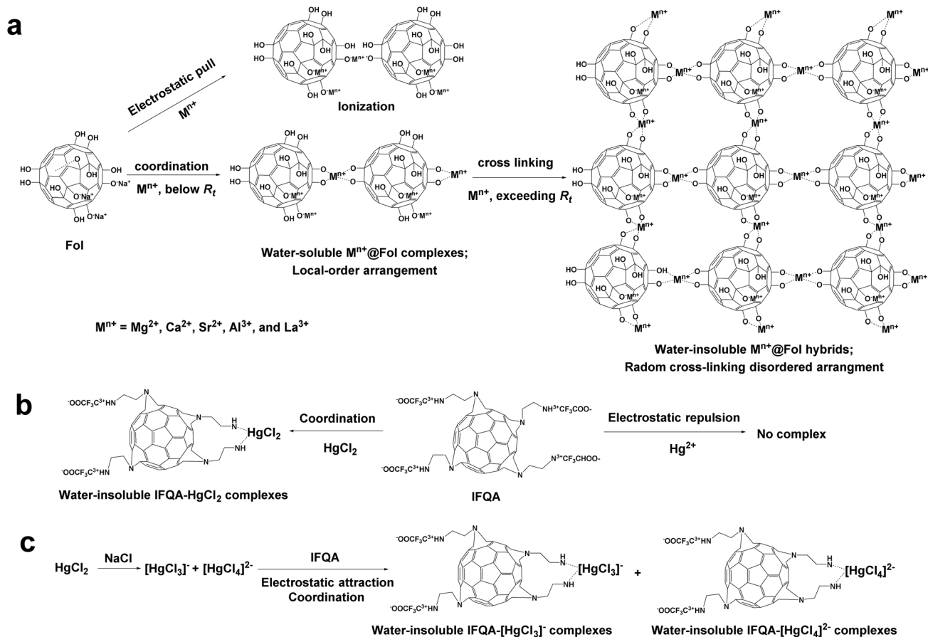
Fig. 10 The scheme of the mode of actions to drive metal-containing ions and water-soluble derivatives of fullerenes for complexation. (a) \text{MCl}_n -Fol solutions; (b) \text{HgCl}_2 -IFQA solution; (c) \text{HgCl}_2 -NaCl-IFQA solution.
