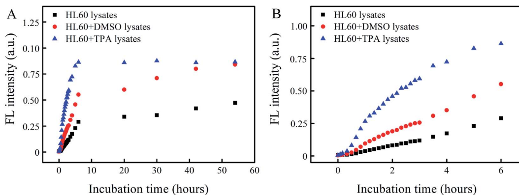
Fig. 4 FL intensities of Abz-FRFK-Dnp@PLGA ( 10 \mu\text{g mL}^{-1} ) incubated with HL60, HL60 + DMSO (granulocyte) and HL60 + TPA (macrophage) lysates as a function of incubation time for comparison of proteolysis rate: (A) up to 54 hours; (B) up to 6 hours.
