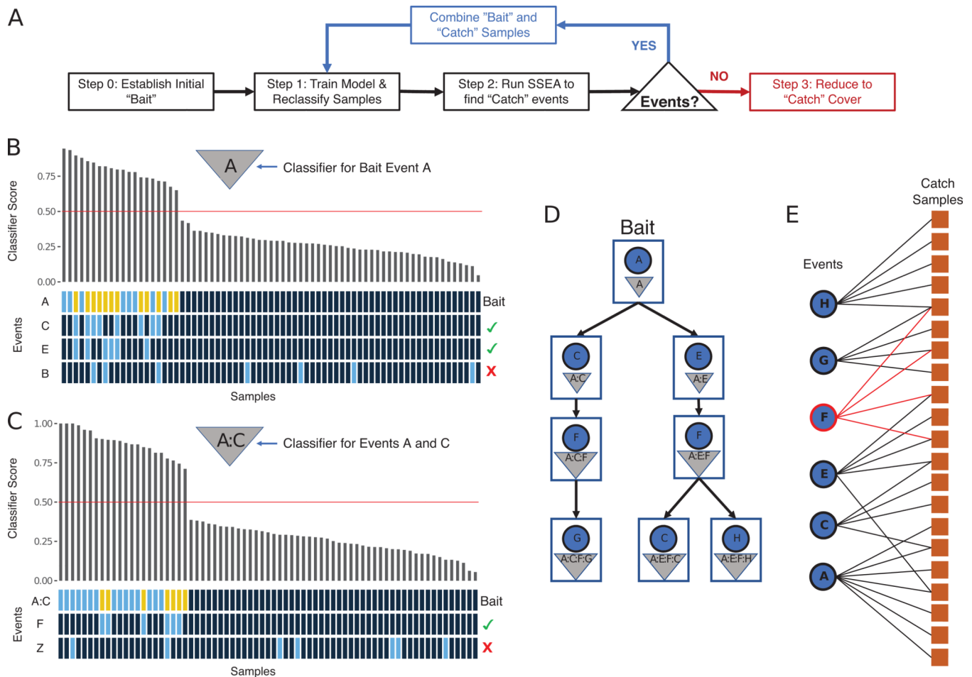
Fig. 1. LURE Method Overview.
