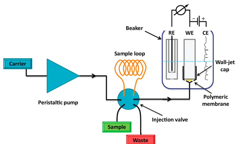
Figure 1. Schematic diagram of the flow-injection system coupled with polyion selective polymeric membrane-based pulstrode used for the experiments reported.
