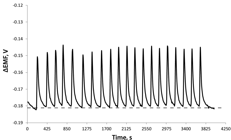
Figure 6. Dynamic potentiometric response to repeated injections ( n = 20 ) of 60 \mu\text{g}/\text{mL} protamine in 10 mM phosphate buffer, pH 7.4, containing 100 mM NaCl. A sampling rate of approximately 20 samples per hour has been achieved. For data shown, the average \Delta\text{EMF} = 33.7 \text{ mV} \pm 1.42 \text{ mV} ( n = 20 ). Flow rate was set at 0.93 mL/min.
