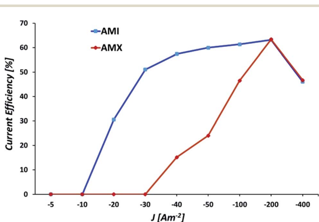
Fig. 16 Current efficiencies for manganese deposition at -5 , -10 , -20 , -30 , -40 , -50 , -100 , -200 , and -400 \text{A m}^{-2} for the AMI 7001s and Neosepta AMX membranes.
