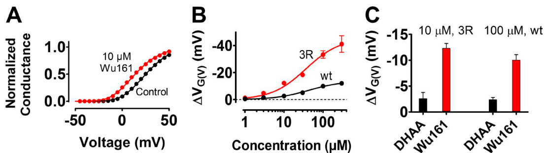
Figure 8. Wu161(p3) is five times more potent than DHAA. (A) Normalized G(V) curves. G(V) shift = -12.4 \text{ mV} . The 3R Shaker K_V channel. pH = 7.4. (B) Concentration-response curves for Wu161(p3). pH = 7.4. Mean \pm SEM ( n = 3-6 ). c_{1/2} = 44 \mu\text{M} , \Delta V_{\text{Max}} = -13.9 \text{ mV} (WT, Eq. 3). c_{1/2} = 36 \mu\text{M} , \Delta V_{\text{Max}} = -45.5 \text{ mV} (3R, Eq. 3). (C) Wu161 and DHAA on the 3R (10 \mu\text{M} ) and WT (100 \mu\text{M} ) Shaker K_V channels, respectively. pH = 7.4. Mean \pm SEM ( n = 3-10 ). Data for DHAA from Ottosson et al. (2015).
