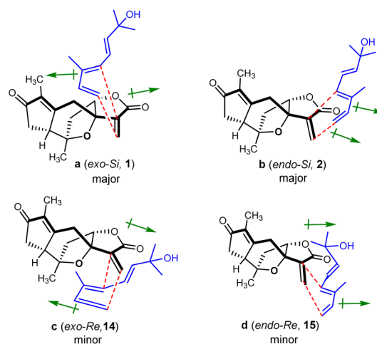
Fig. 3 Transition states proposed for the regio-specific intermolecular Diels–Alder reactions of 4 and 5 ( \leftrightarrow : denotes dipole moments of the dienophile enone and diene systems).
