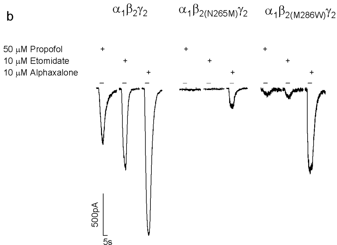
Direct activation of \alpha_1\beta_2\gamma_2 GABA A receptors by intravenous general anesthetics. (a) Bar histogram of the direct activation of GABA A receptor-mediated chloride currents by propofol, etomidate and alphaxalone. Data points represent means \pm standard error, n = 9–19; *p < 0.05; Student's t-test). (b) Selected traces showing representative whole-cell chloride currents activated by propofol, etomidate and alphaxalone.
