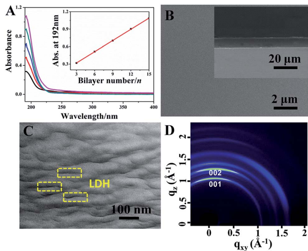
Fig. 3 (A) UV-vis absorption spectra of the (LDH-80/PDMS) _n ( n = 3-15 ) films on quartz glass substrates (inset: the linear relationship between absorbance at 192 nm and bilayer number n ); (B) top-view and side-view (inset) SEM images of (LDH-80/PDMS) _{15} film; (C) side-view TEM image and (D) 2D grazing-incidence XRD patterns for (LDH-80/PDMS) _{15} film.
