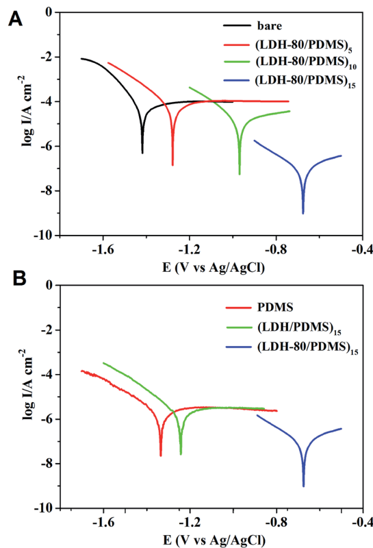
Fig. 7 (A) Potentiodynamic polarization curves of bare Al substrate, (LDH-80/PDMS) n films on Al substrate with n = 5, 10 and 15; (B) Potentiodynamic polarization curves of PDMS, (LDH/PDMS) 15 and (LDH-80/PDMS) 15 film, respectively.
