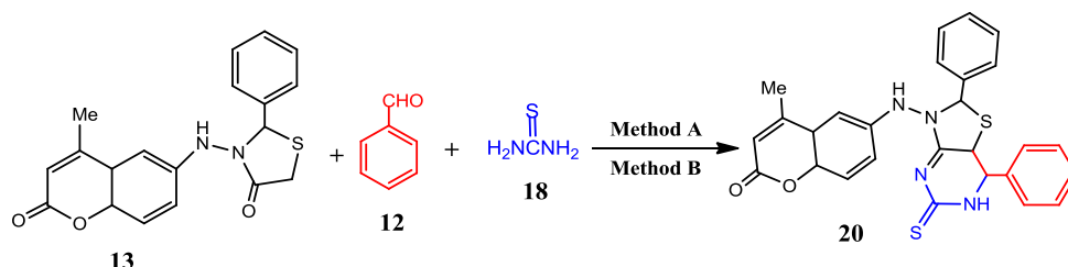
Scheme 8. Synthesis of 2,7-diphenyl-5-thioxothiazolo[4,5- d ]pyrimidine derivative 20 .
