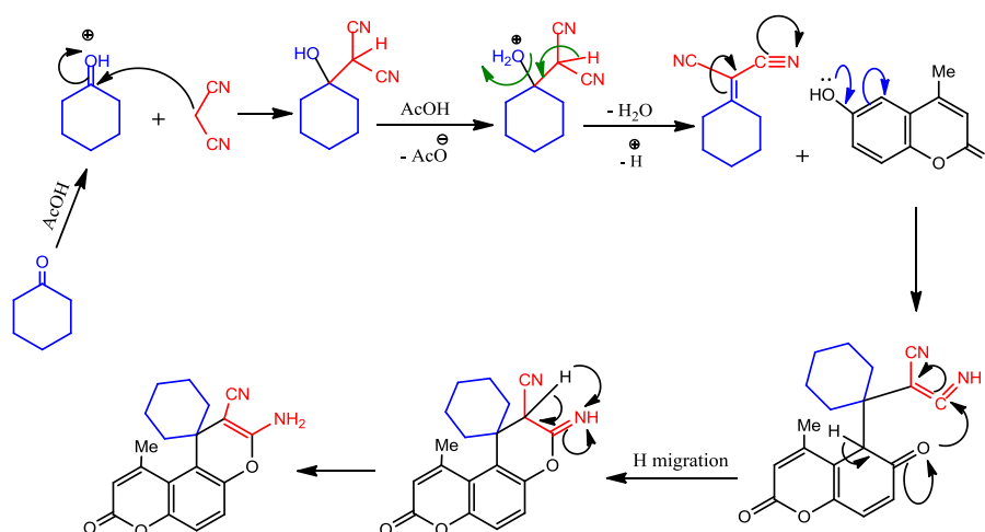
Chart 1. Mechanistic pathway of 3'-amino-10'-methyl-8'-oxo-8' H -spiro-[cyclohexane-1,1'-pyrano-[3,2- f ]chromene]-2'-carbonitrile 8b .
