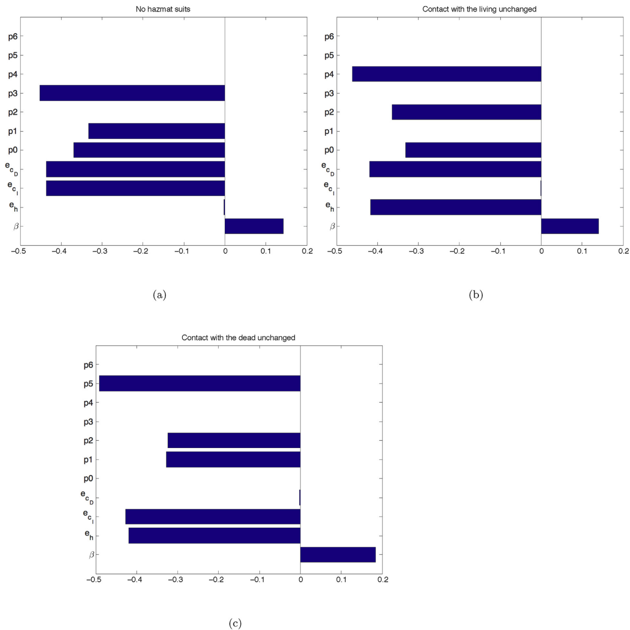
Fig. 8. PRCCs for some possibilities outside the ranges in Table 1: (a) the absence of hazmat suits, (b) when contact with the living infected is unchanged and (c) when contact with dead bodies is unchanged. In each case, the most significant influence on the outcome is the combination of the remaining protection protocols, followed by the efficacies of those remaining protection protocols.
