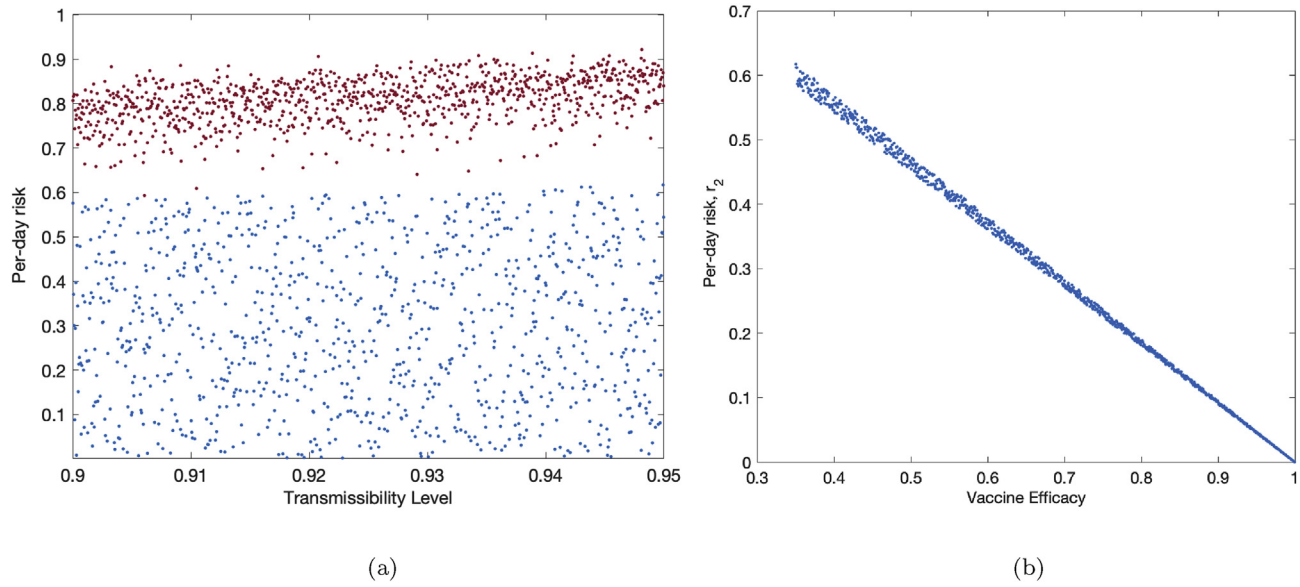
Fig. 4. Sensitivity of the daily risk of Ebola to transmission rates and vaccine efficacy when all susceptible individuals get vaccinated. The red dots represent the current risk of infection while the blue dots represent the post-vaccine risk of Ebola. This is an ideal case, and the proportion of use of the vaccine q_7 is set to 1. The transmission rate \beta is between 0.9 and 0.95.
