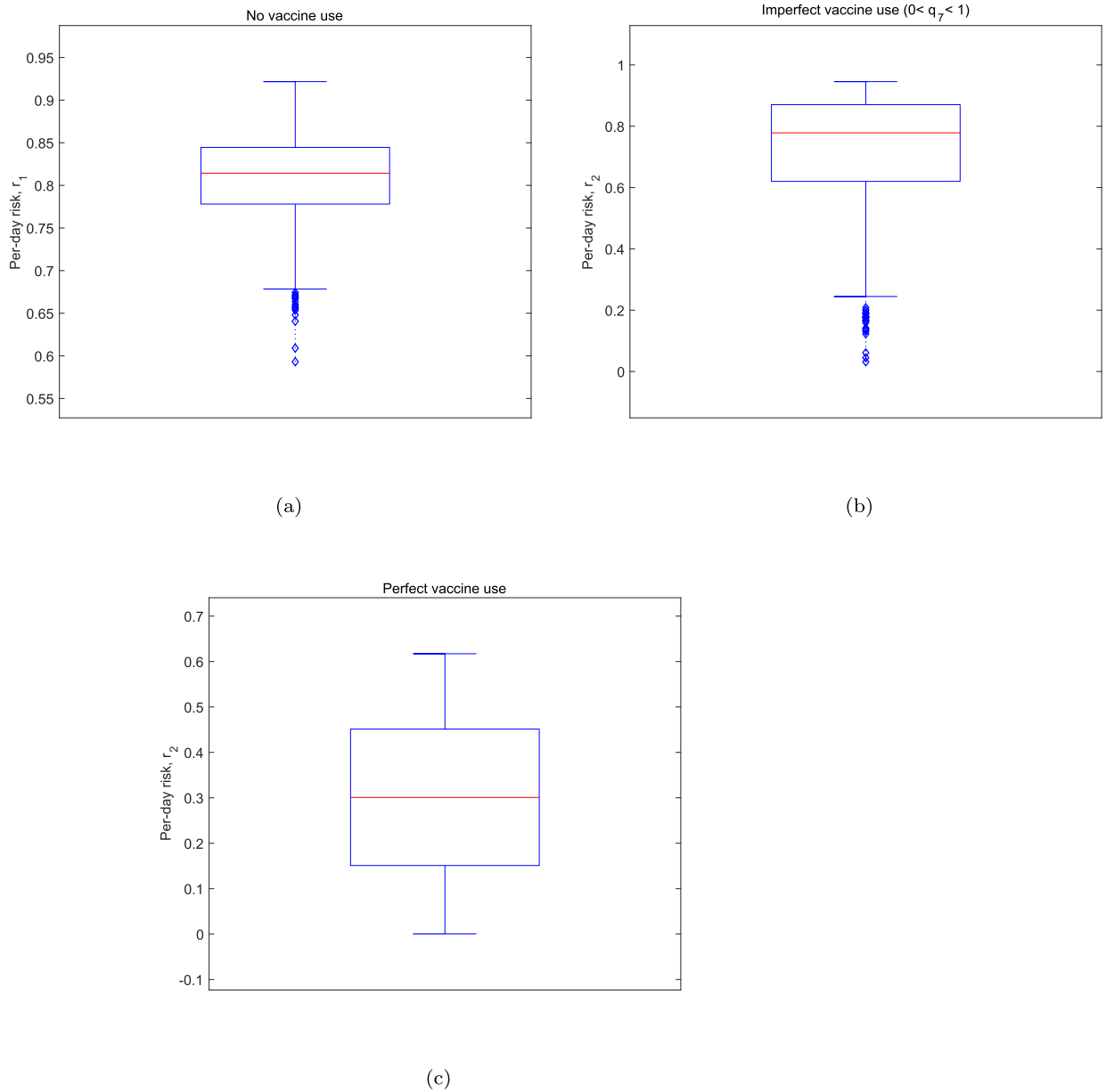
Fig. 5. Boxplots of 1000 sampled values using the LHS ranges from Table 1. The horizontal red line indicates the median value. We present the daily risk of Ebola under three scenarios: before the vaccine, imperfect vaccine uptake ( 0 < q_7 < 1 ) and perfect vaccine use ( q_7 = 1 ).
