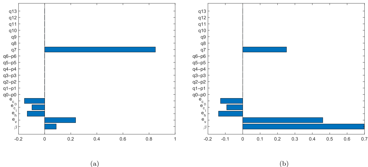
Fig. 6. PRCCs for parameters that affect r^* . (a) The case for general vaccine uptake ( 0 < q_7 < 1 ). (b) The case for high vaccine uptake ( 0.7 < q_7 < 1 ). The transmission rate \beta is between 0.5 and 1.
