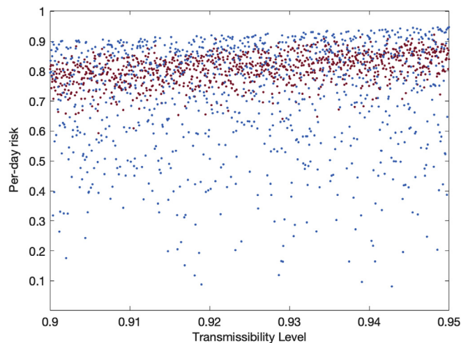
Fig. 2. Sensitivity of the daily risk of Ebola to transmission rates when the only protection protocol available is the vaccine. The red dots represent the current daily risk of infection while the blue dots represent the post-vaccine daily risk of contamination. The proportional vaccine uptake q_7 ranges from 0 to 1 and the transmission rate \beta is between 0.9 and 0.95.
