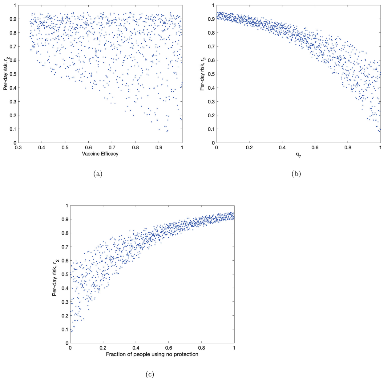
Fig. 3. Sensitivity of the daily risk of Ebola to the effectiveness of the vaccine e_v , its proportion of use q_7 and the fraction of people not using any protection. The proportional vaccine uptake q_7 varies from 0 to 1, and vaccination is the only available protection protocol. The transmission rate \beta is between 0.9 and 0.95.
