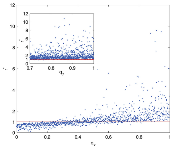
Fig. 7. Sensitivity of the threshold level r^* to (a) the fraction of people using the vaccine q_7 and (b) the fraction of people not using any protection. The transmission rate \beta is between 0.5 and 1. Inset: the range q_7 > 70\% that guarantees risk reduction.
