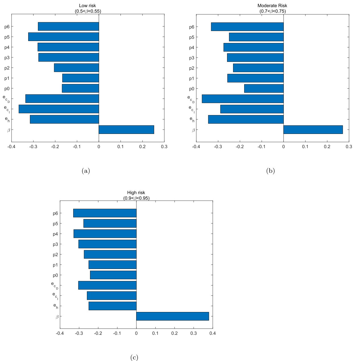
Fig. 1. PRCCs before vaccine introduction for low (50–55%), moderate (70–75%) and high (90–95%) levels of transmissibility. The outcome variable is the daily risk of infection before vaccination, r_1 .
