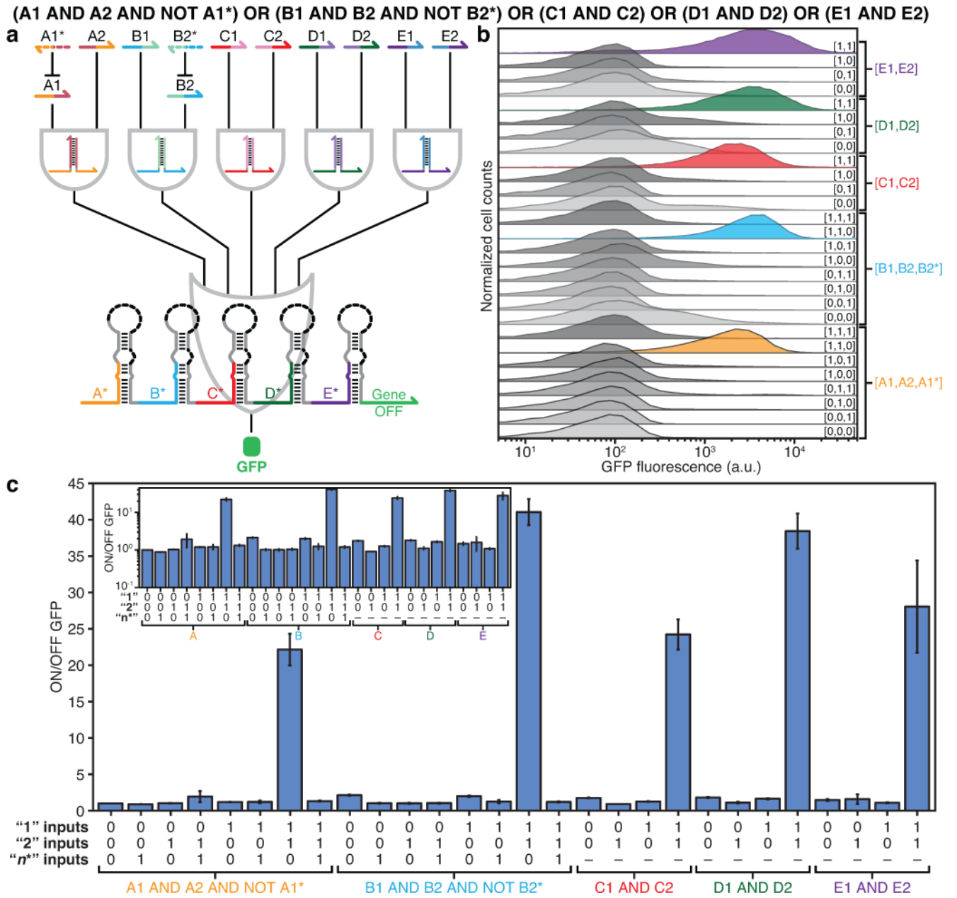
Figure 4. 12-input disjunctive normal form (DNF) ribocomputing circuit
