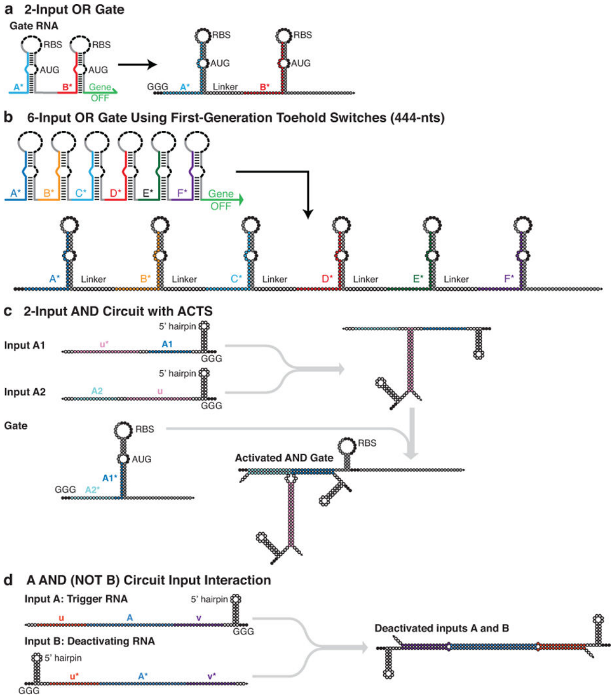
Extended Data Figure 2. Nucleotide-level schematics of ribocomputing devices
