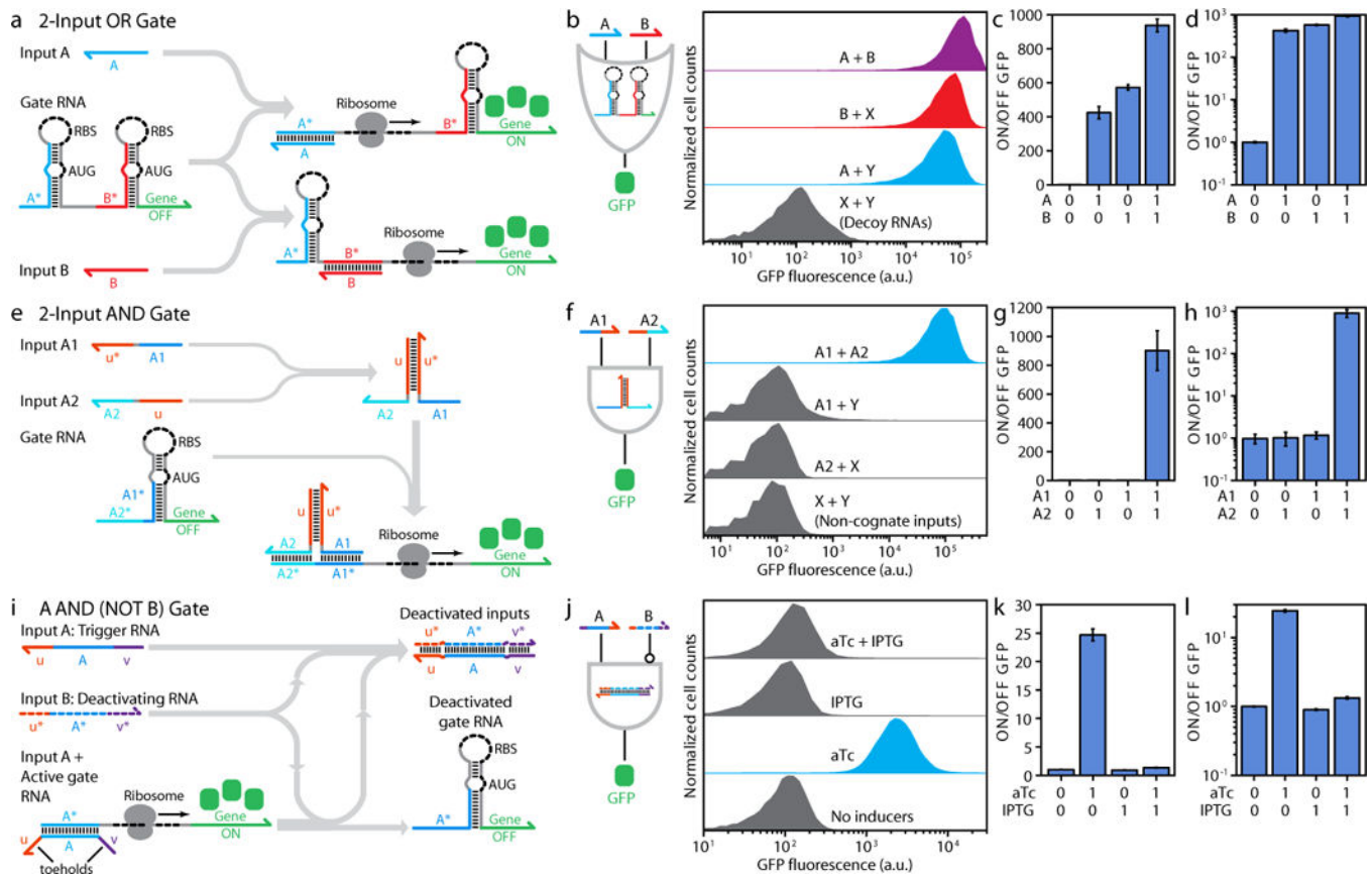
Figure 2. Two-input ribocomputing logic circuits
