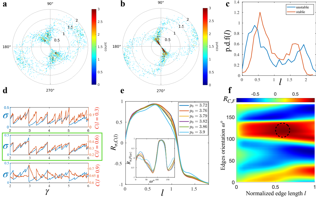
FIG. 2. A new approach to infer tissue stress: (a) Polar distribution of cell edge vectors in a stable state. (b) Polar distribution of cell edge vectors in an unstable state. (c) Edge length density distribution at different instability. Panels (a-c) were created using p_0 = 3.72 . (d) The stress-strain curve is overlaid with C(l) -strain curve at different l . The green box denotes the trace with high correlation between \sigma and C(l) . (e) The correlation between tissue stress and the cumulative edge length distribution R_{\sigma,C(l)} suggests a robust critical normalized edge length l^* . Inset: The correlation between tissue stress and the portion of edges at different orientation R_{\sigma,F(\omega)} . (f) Color-plot of the correlation R_{C,F} between edges length distribution and edges orientation distribution. The black-dashed circle indicates the region in where the correlation is maximized, from which l^* could be determined.
