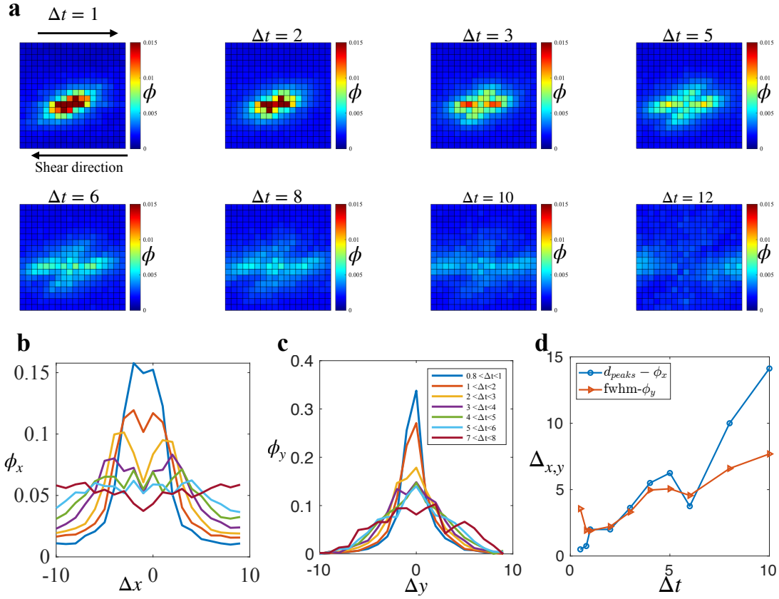
FIG. 4. Propagation of plastic events. (a) Evolution of the probability field \phi at p_0 = 3.72 . Each image corresponds to the probability field at a particular time lag \Delta t . Bright regions indicate a high probability of finding another rearrangement in the region relative to the causal rearrangement. (b) Spatial distribution of the correlation field \phi_x as a function of the relative horizontal position \Delta x . The distribution has a diffusing bimodal shape, indicating a convection process alongside diffusion. (c) Spatial distribution of the correlation field \phi_y as a function of the relative vertical position \Delta y . The distribution is bell-shaped, with the width of the bell increasing as time progresses, indicating a pure diffusion process. (d) The separation of the peaks in \phi_x and the Full Width at Half Maximum (FWHM) of \phi_y as functions of the time lag \Delta t .
