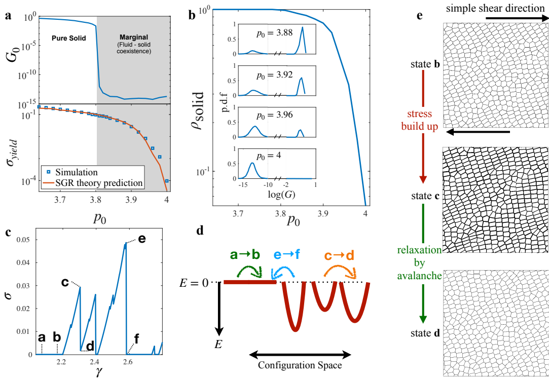
FIG. 1. (a) Discrepancy between shear start-up and steady-shear regime. Top: The shear modulus of the un-sheared tissue ( \gamma = 0 ). The shear modulus is obtained using linear-response calculation (see Methods). Bottom: The yield stress \sigma_{yield} obtained from the steady-state shear regime of quasi-static simulations is shown together with the yield stress obtained from the SGR model, where the only fitting parameter in the model, the elastic constant of an element was chosen to be k = 0.0386 . (b) The probability of finding the system in solid state as a function of p_0 . Inset: Distribution of tissue stress at different p_0 . (c) Stress-strain curve example showing different yielding types: a fluid state yields to another fluid states a \rightarrow b , a solid state yields to another solid one c \rightarrow d , and a solid state yields to a fluid state e \rightarrow f . (d) Schematic of the dynamics of elements in the SGR model: The energy landscape of the material consists of traps with different depth E drawn from a distribution \rho(E) that characterizes the structural disorder of the material. Yielding events are captured by transitions from one trap to another. The three types of transition illustrates the transitions observed in simulation. (e) Simulation snapshots at different stages of a stress build-up and relaxation process. The edge thickness represents the edge tension, with thicker edges indicating higher tension. Here the states correspond to the ones labeled in panel e.
