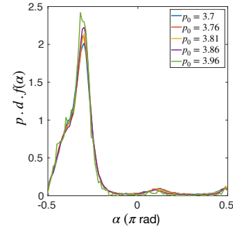
FIG. S4. The orientation distribution of T1-edges (edges undergo T1 transitions) at various values of p_0 .
