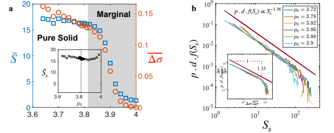
FIG. 5. Avalanches statistics. (a) Dependence of average yielding size \bar{S} and average stress relaxed \Delta\sigma on p_0 . Inset: Dependence of average avalanche size \bar{S}_s on p_0 . (b) Distribution of avalanche size follows a power-law distribution. Inset: Distribution of scaled average stress relaxed by avalanches also follows the same power law
