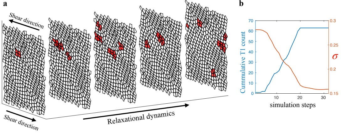
FIG. 3. Spatiotemporal map of plastic events in tissue. (a) Space-time map of plastics rearrangement in the form of T1 transition during an avalanche. Cells that participated in T1 transitions are labeled in red. The example avalanche was selected from a system at p_0 = 3.72 . (b) Number of accumulative plastic rearrangement and tissue shear stress as the avalanche progresses.
