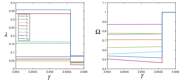
FIG. S3. Evolution of low-frequency mode near avalanches.
