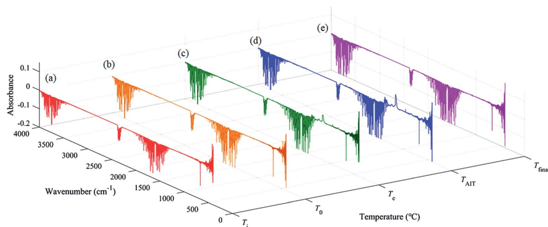
Fig. 9 FTIR spectra of the evolved gas for [EMIM][Tf 2 N] heated in nitrogen atmosphere. The wave numbers ranged from 400–4000 \text{cm}^{-1} . The FTIR spectra were collected at five different temperatures: (a) ambient temperature ( T_i ); (b) onset temperature ( T_0 ); (c) estimated onset temperature ( T_e ) from TGA curve; (d) auto-ignition temperature ( T_{AIT} ); (e) temperature at the termination of the test ( T_{final} ).
