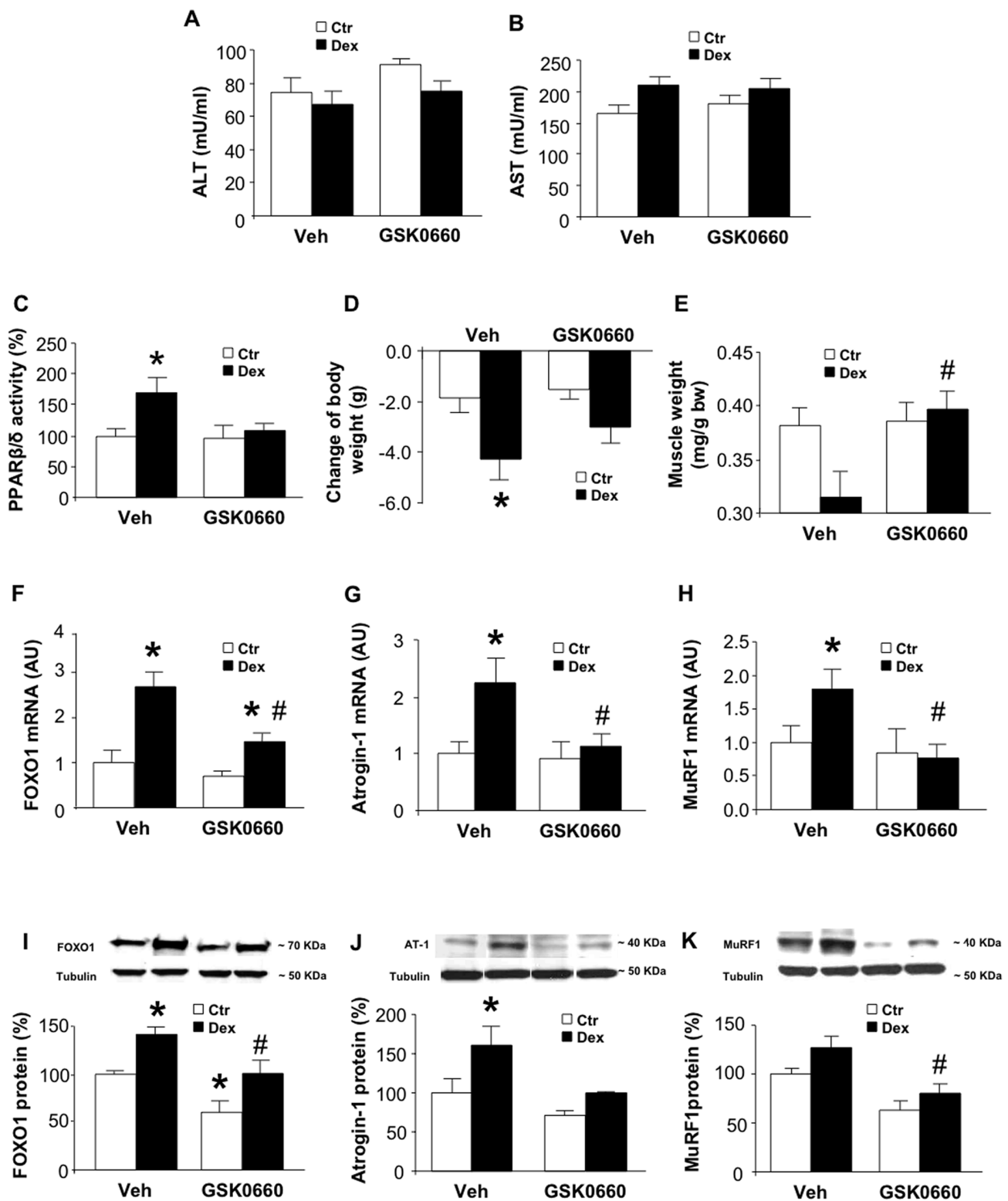
Figure 6. Treatment of rats with GSK0660 prevents dexamethasone-induced muscle wasting. A) and B) Serum ALT and AST levels in control and dexamethasone-treated (10 mg/kg) rats that were administered vehicle or GSK0660 (1 mg/kg). C) PPAR \beta/\delta activity in EDL muscles from control and dexamethasone-treated rats that were administered vehicle or GSK0660. D) Change of body weight in control and dexamethasone-treated rats that were administered vehicle or GSK0660. E) Muscle weight in control and dexamethasone-treated rats that were administered vehicle or GSK0660. F-H) mRNA and I-K) protein levels for FOXO1, atrogin-1, and MuRF1 in muscles from control and dexamethasone-treated rats that were administered vehicle or GSK0660. Results are means \pm SEM with n=8 /group. * p<0.05 vs appropriate control group; # p<0.05 vs Veh/Dex group by ANOVA.
