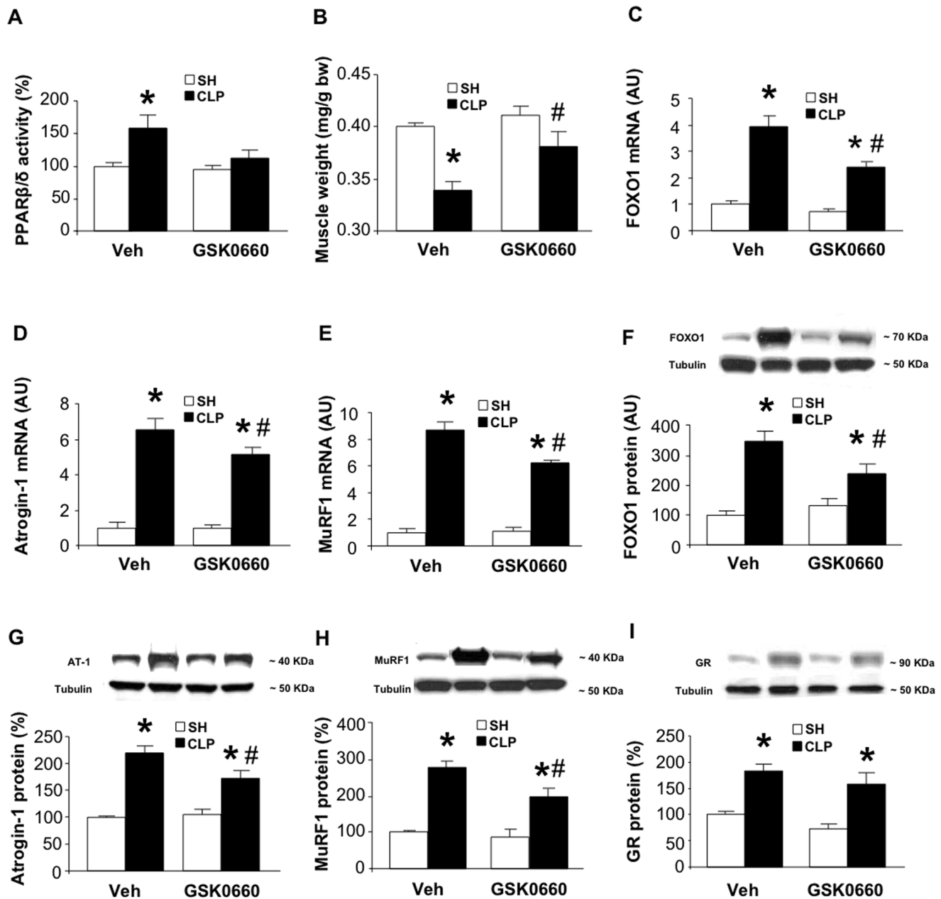
Figure 8. Sepsis-induced muscle wasting in rats is improved by treatment with GSK0660. A) PPAR \beta/\delta activity in EDL muscles from sham-operated (SH) and septic (CLP) rats treated with vehicle or GSK0660 (1 mg/kg). B) Muscle weight in sham-operated and septic rats treated with vehicle or GSK0660. C-E) mRNA and F-H) protein levels for FOXO1, atrogin-1, and MuRF1 in muscles from sham-operated and septic rats treated with vehicle or GSK0660. I) GR protein levels in EDL muscles from sham-operated and septic rats treated with vehicle or GSK0660. Results are means \pm SEM with n=8 /group except in panel I where n=4 /group. * p<0.05 vs appropriate sham group; # p<0.05 vs Veh/CLP by ANOVA. doi:10.1371/journal.pone.0059726.g008
