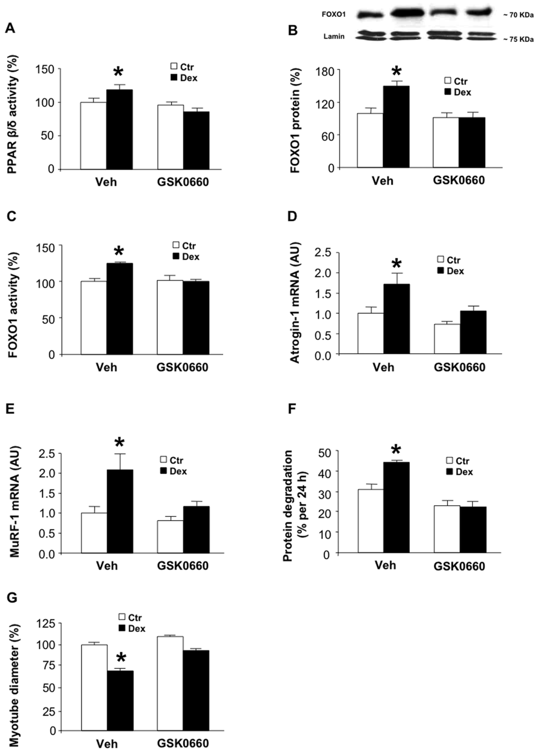
Figure 4. The PPAR \beta/\delta antagonist GSK0660 blocks the catabolic effects of dexamethasone in cultured L6 myotubes. A) PPAR \beta/\delta activity in myotubes treated with or without 1 \mu M dexamethasone in the absence or presence of 0.1 \mu M GSK0660. B) FOXO1 protein levels in myotubes treated as described in panel A. FOXO1 levels were determined by Western blotting of nuclear extracts and A/C lamin levels were determined as loading controls. C) FOXO1 activity in myotubes treated for 24 h with 1 \mu M dexamethasone in the absence or presence of 0.1 \mu M GSK0660. D) Atrogin-1 and E) MuRF1 mRNA levels in myotubes treated for 24 h with or without 1 \mu M dexamethasone in the absence or presence of 0.1 \mu M GSK0660. F) Protein degradation (% per 24 h) in myotubes treated for 24 h with or without 1 \mu M dexamethasone in the absence or presence of 0.1 \mu M GSK0660. G) Diameter of myotubes after treatment for 24 h with or without 1 \mu M dexamethasone in the absence or presence of 0.1 \mu M GSK0660. Results are means \pm SEM with n=7 or 8/group. *p<0.05 vs Ctr/Veh by ANOVA. doi:10.1371/journal.pone.0059726.g004
