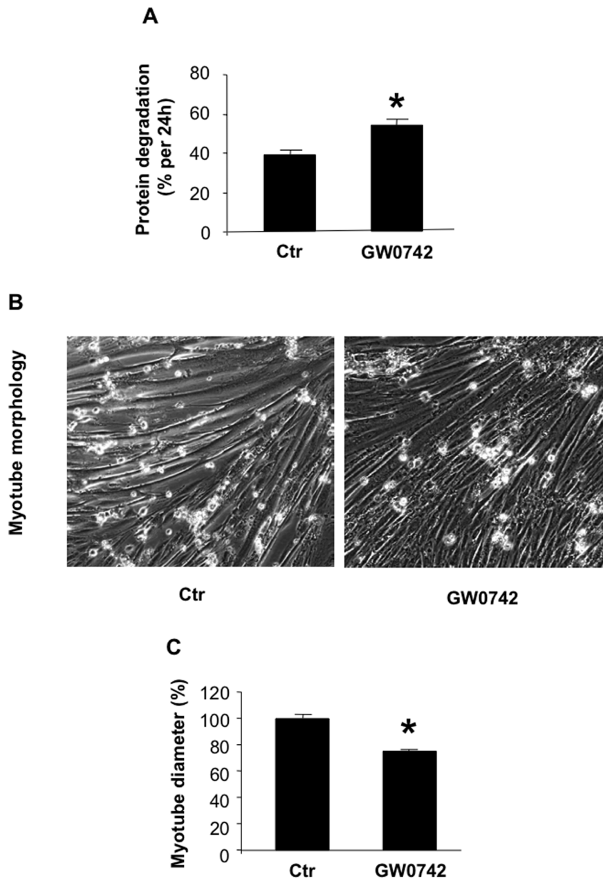
Figure 2. The PPAR \beta/\delta agonist GW0742 increases protein degradation and induces atrophy of cultured L6 myotubes. A) Protein degradation (% per 24 h) in myotubes treated for 24 h with 0.1 \mu M GW0742 or vehicle (Ctr). B) Morphology of cultured L6 myotubes after treatment for 24 h with 0.1 \mu M GW0742 or vehicle (Ctr). Myotubes were photographed under a phase contrast microscope at 100 \times magnification. C) Diameter of cultured myotubes after treatment for 24 h with 0.1 \mu M GW0742 or vehicle (Ctr). Results are means \pm SEM with n=8 /group.* p<0.05 vs control. doi:10.1371/journal.pone.0059726.g002
