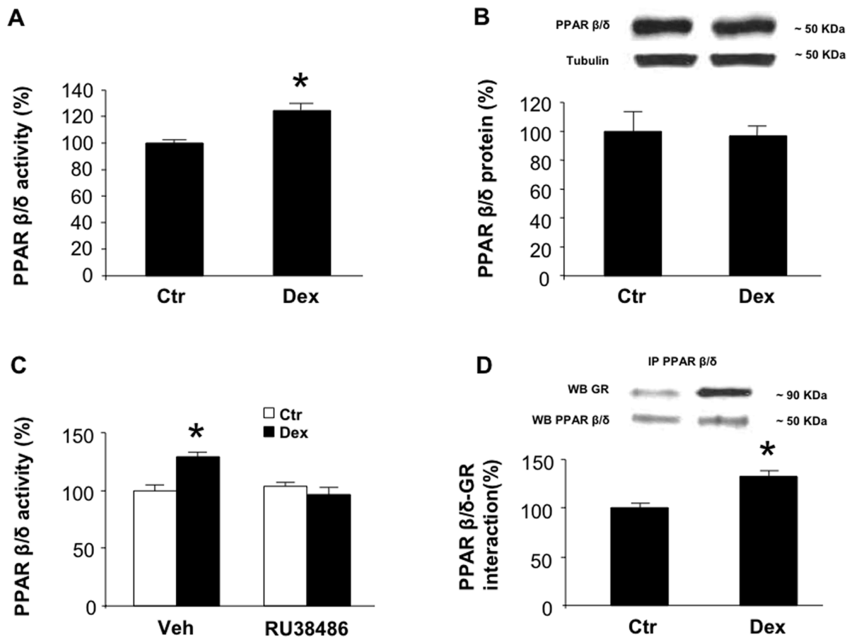
Figure 3. Dexamethasone increases PPAR \beta/\delta activity in cultured L6 myotubes through a GR-dependent mechanism. A) PPAR \beta/\delta activity in myotubes treated for 24 h with 1 \mu M dexamethasone or vehicle (Ctr). Results are expressed as percent of control. B) PPAR \beta/\delta protein levels determined by Western blotting in total cell lysates from control and dexamethasone-treated myotubes. Representative Western blots are shown in the upper panel and densitometric quantifications in the lower panel. \alpha -Tubulin was determined for loading control. C) PPAR \beta/\delta activity in control and dexamethasone-treated myotubes. Myotubes were treated for 24 h with dexamethasone (1 \mu M) in the absence or presence of 10 \mu M RU38486. D) PPAR \beta/\delta -GR interaction determined by co-immunoprecipitation of myotube proteins extracted from whole cell lysates after treatment of the myotubes for 24 h with 1 \mu M dexamethasone or vehicle (Ctr). A PPAR \beta/\delta antibody was used for pull-down followed by immunoblotting with a GR or PPAR \beta/\delta antibody. Representative immunoblots are shown in the upper panel and densitometric quantifications of the upper bands in the immunoblots are shown in the lower panel. Results were calculated as percent of control and are means \pm SEM with n=7 or 8 /group. * p<0.05 vs Ctr by Student's t-test (panel A and D) or ANOVA (panel C). doi:10.1371/journal.pone.0059726.g003
