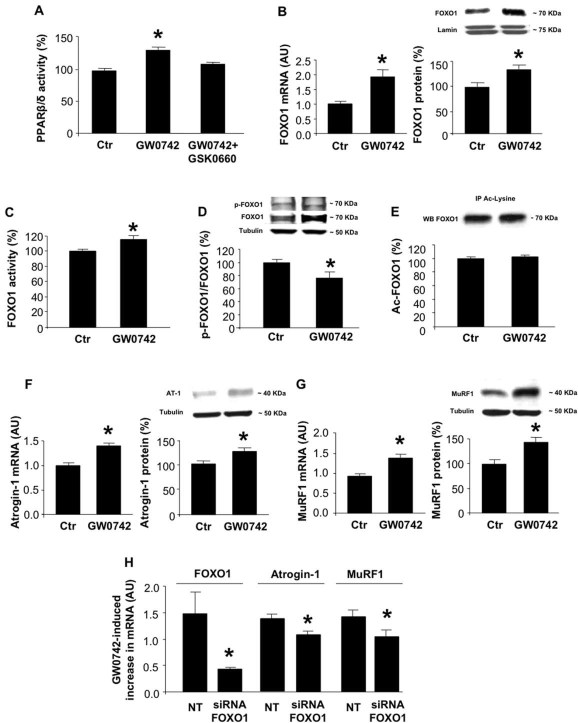
Figure 1. PPAR \beta/\delta activation upregulates atrogen-1 and MuRF1 expression through a FOXO1-dependent mechanism in L6 myotubes. A) PPAR \beta/\delta activity in cultured L6 myotubes treated for 24 h with 0.1 \mu M GW0742 in the absence or presence of 0.1 \mu M GSK0660. Results are expressed as percent of control (Ctr). B) FOXO1 mRNA (left panel) and protein levels (right panel) in cultured L6 myotubes after treatment for 24 h with 0.1 \mu M GW0742. Representative Western blots are shown in the upper and densitometric quantifications in the lower panel. A/C lamin was determined for loading control. C) FOXO1 DNA binding activity in control and GW0742-treated myotubes. D) p-FOXO1(Ser 256) and total FOXO1 protein levels (upper panel) and calculated p-FOXO1/FOXO1 ratio in cultured L6 myotubes after treatment for 24 h with 0.1 \mu M GW0742. The calculated p-FOXO1/FOXO1 ratio was based on densitometric quantifications of p-FOXO1 and total FOXO1 levels on Western blots. E) Ac-FOXO1 levels in control and GW0742-treated myotubes determined by co-immunoprecipitation. F) Atrogen-1 mRNA and protein levels in cultured L6 myotubes after treatment for 24 h with 0.1 \mu M GW0742 and in control myotubes. \alpha -Tubulin was determined for loading control. G) MuRF1 mRNA and protein levels in control and GW0742-treated myotubes. H) GW0742-induced increase in mRNA levels for FOXO1, atrogen-1, and MuRF1 in myotubes transfected with a non-targeting (NT) or FOXO1 siRNA. Results are means \pm SEM with n=7 or 8/group. *p<0.05 vs control (Ctr) or NT groups by Student's t-test (panel B-H) or ANOVA (panel A). doi:10.1371/journal.pone.0059726.g001
