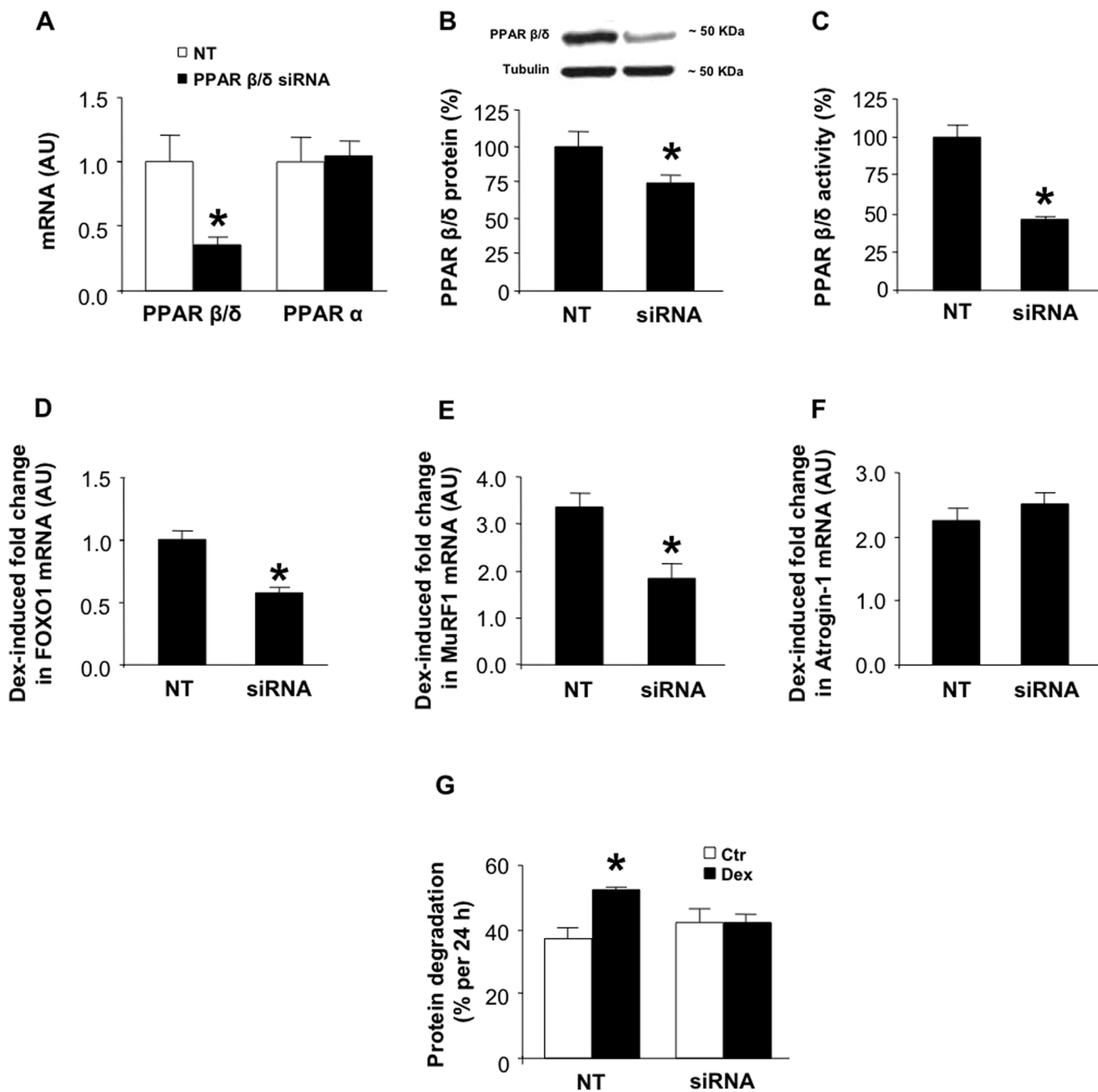
Figure 5. Downregulation of PPAR \beta/\delta expression reduces FOXO1 and MuRF1 expression and protein degradation in dexamethasone-treated myotubes. A) mRNA levels for PPAR \beta/\delta and PPAR \alpha in myotubes transfected with non-targeting (NT) or PPAR \beta/\delta siRNA. B) PPAR \beta/\delta protein levels in myotubes transfected with non-targeting (NT) or PPAR \beta/\delta siRNA. Representative Western blots are shown in the upper and densitometric quantifications in the lower panel. C) PPAR \beta/\delta activity in myotubes transfected with non-targeting (NT) or PPAR \beta/\delta siRNA. D–F) Dexamethasone-induced changes in FOXO1, MuRF1, and atrogin-1 mRNA in myotubes transfected with non-targeting (NT) or PPAR \beta/\delta siRNA. G) Protein degradation in myotubes treated for 24 h with or without 1 \mu M dexamethasone following transfection with non-targeting (NT) or PPAR \beta/\delta siRNA. Results are reported as arbitrary units (AU) or percent of control and are means \pm SEM with n=7 or 8/group. *p<0.05 vs appropriate control group by ANOVA (panel G) or Student's t-test. doi:10.1371/journal.pone.0059726.g005
