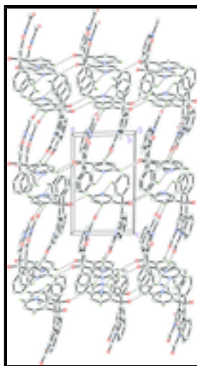
Fig. 2. The crystal structure of the title compound, viewed along the b axis, showing a three-dimensional framework. H atoms not involved in intermolecular interactions (dashed lines) have been omitted for clarity.
