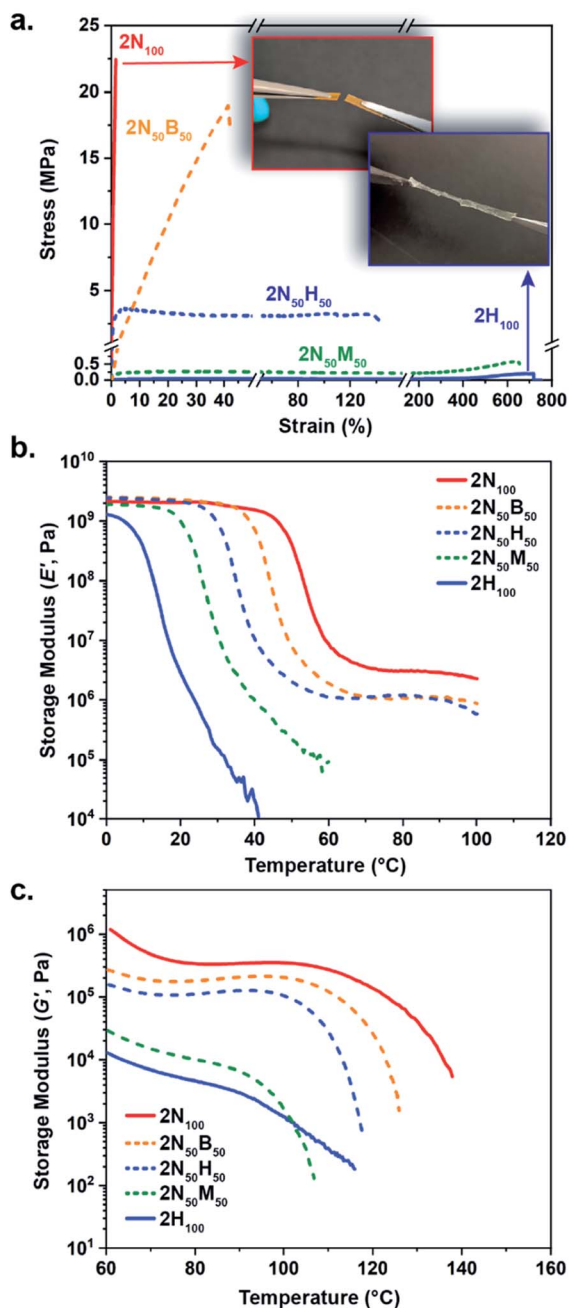
Fig. 4 (a) Stress–strain curves (strain rate = 10 \text{ mm min}^{-1} , 25 \text{ }^\circ\text{C} ), (b) dynamic mechanical analysis (DMA; temperature ramp rate = 3 \text{ }^\circ\text{C min}^{-1} , frequency = 1 \text{ Hz} , tensile geometry) and (c) shear rheology (temperature ramp rate = 3 \text{ }^\circ\text{C min}^{-1} , frequency = 2 \text{ Hz} , parallel plate geometry) curves for 2\text{N}_{100} (red), 2\text{N}_{50}\text{B}_{50} (dashed orange), 2\text{N}_{50}\text{H}_{50} (dashed blue), 2\text{N}_{50}\text{M}_{50} (dashed green), and 2\text{H}_{100} (blue).
