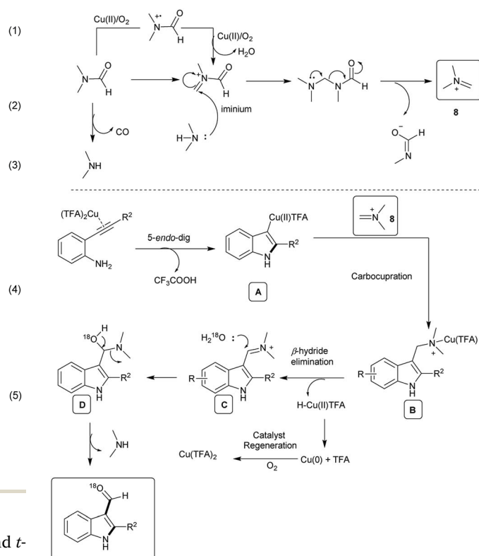
Scheme 6 Proposed mechanism.
