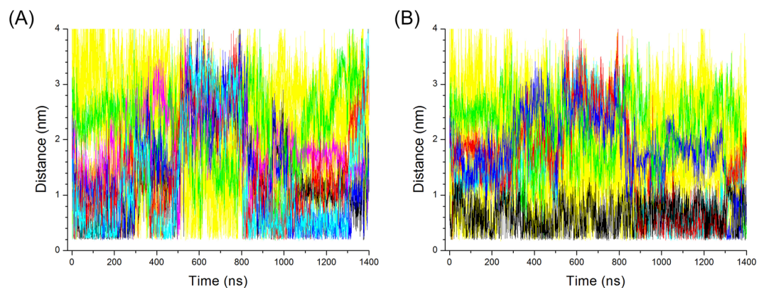
Figure 6. Trajectories of changes in the distance of salt bridges of Lys87 and Arg88 in Ec0VV_6A during 1400 ns at 450 K. (A) Salt bridges of Lys87: Lys87-Asp20 (black), Lys87-Asp26 (magenta), Lys87-Asp39 (green), Lys87-Glu21 (blue), Lys87-Glu57 (red), Lys87-Glu59 (cyan), and Lys87-others (yellow). (B) Salt bridges of Arg88: Arg88-Asp20 (cyan), Arg88-Glu21 (red), Arg88-Asp26 (blue), Arg88-Asp39 (green), Arg88-Glu90 (black), and Arg88-others (yellow).
