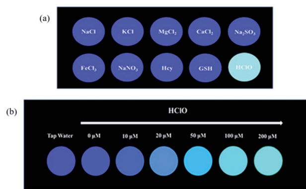
Fig. 8 (a) Fluorescence images of test paper soaked with probe BNA-HClO to detection interfering substances ( 1 \text{ mmol L}^{-1} ) and HClO ( 100 \mu\text{mol L}^{-1} ) under 365 nm, (b) fluorescence images of test paper soaked with probe BNA-HClO to detection HClO ( 0\text{--}200 \mu\text{mol L}^{-1} ) in water under 365 nm.
