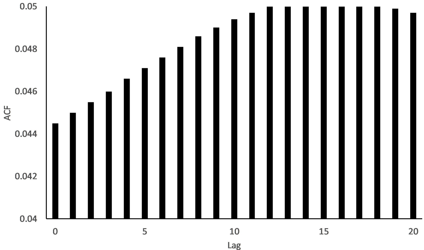
Fig 3. Cross-correlation between tide height and depth measured at the 250m below bund location. Maximum correlation occurs at a lag of 12 to 17 which is equivalent to a 3 to 4.25 hr delay between tides experienced at the coast and measured changes in depth at the 250m below bund location— 15 min data records. 95% CI has been omitted from the graph falling at \pm 0.05 .
