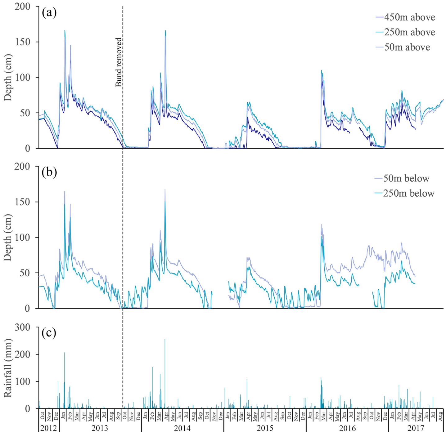
Fig 2. Changes in depth above and below the bund location and daily rainfall—October 2012 to August 2017. Logger distances above the bund (a) are 450 m, 250 m and 50 m and below (b) are 50 m and 250 m. The bund was removed on the 6 th October 2013. Daily rainfall (c) was derived from the nearby Bureau of Meteorology station at Allingham approximately 2.5 km distant.
