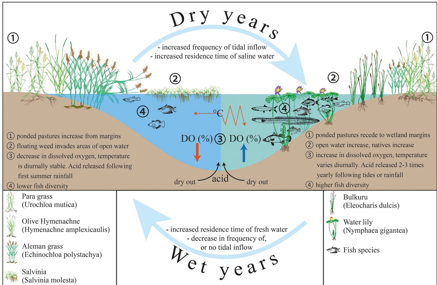
Fig 19. Conceptual model showing changes due to seasonal oscillations within the shallow Boolgooroo region of the Mungalla wetlands. This oscillation/cycle is likely to occur on other shallow wetlands if this method of passive remediation is employed.
