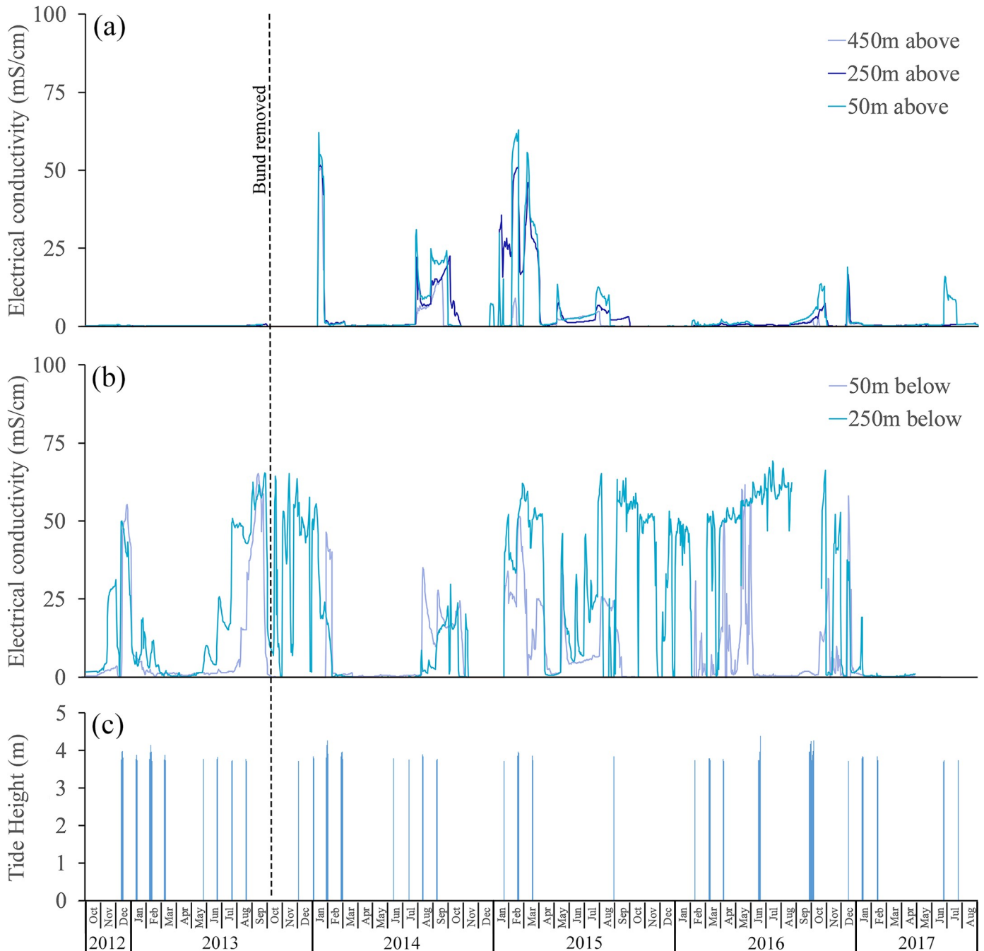
Fig 4. Changes in salinity above and below the bund location and tides \geq 3.6 m—October 2012 to August 2017. Logger distances above the bund are 450 m, 250 m and 50 m and below are 50 m and 250 m. The bund was removed on the 6th October 2013. High tides ( \geq 3.6 m) are for Forrest Beach.
