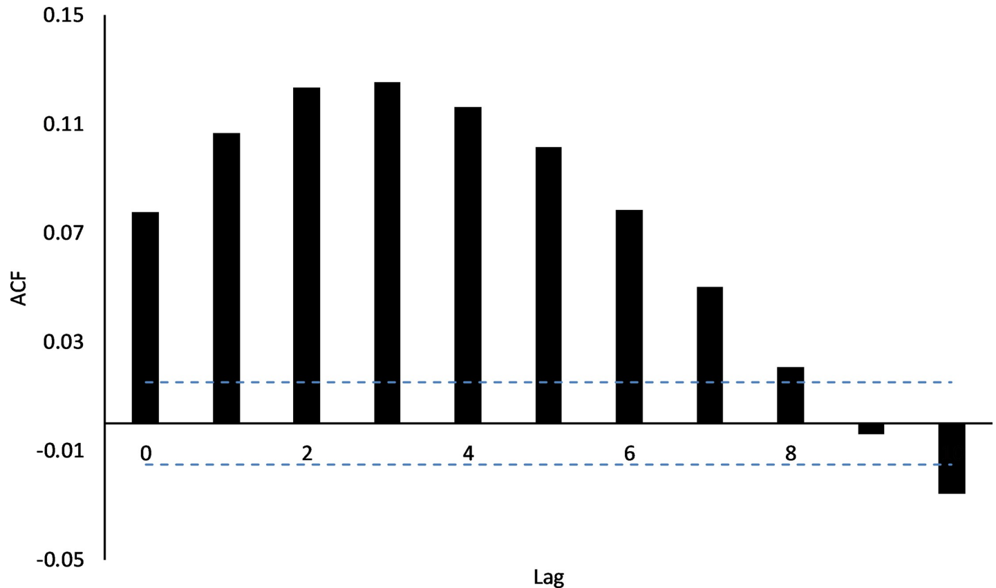
Fig 6. Cross-correlation between tide height and EC measured at the 50m above bund location. Maximum correlation occurs at a lag of 3 which is equivalent to a 3-day delay between tides experienced at the coast and measured changes in EC.
