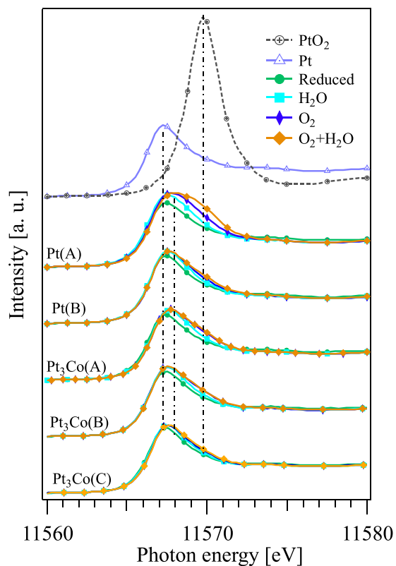
Figure 4. In situ HERFD-XAS spectra of Pt and Pt_3Co nanoparticles under reduced condition, O_2 , H_2O , as well as O_2 + H_2O adsorptions for Pt(A), Pt(B), Pt_3Co (A), Pt_3Co (B), Pt_3Co (C) samples from top to the bottom. HERFD-XAS spectra of the Pt foil and PtO_2 powder were also shown as standards of fully reduced and oxidized conditions. The vertical dotted-broken lines are drawn to the peak positions of Pt foil, PtO_2 , and Pt(A) under O_2 + H_2O adsorption.
