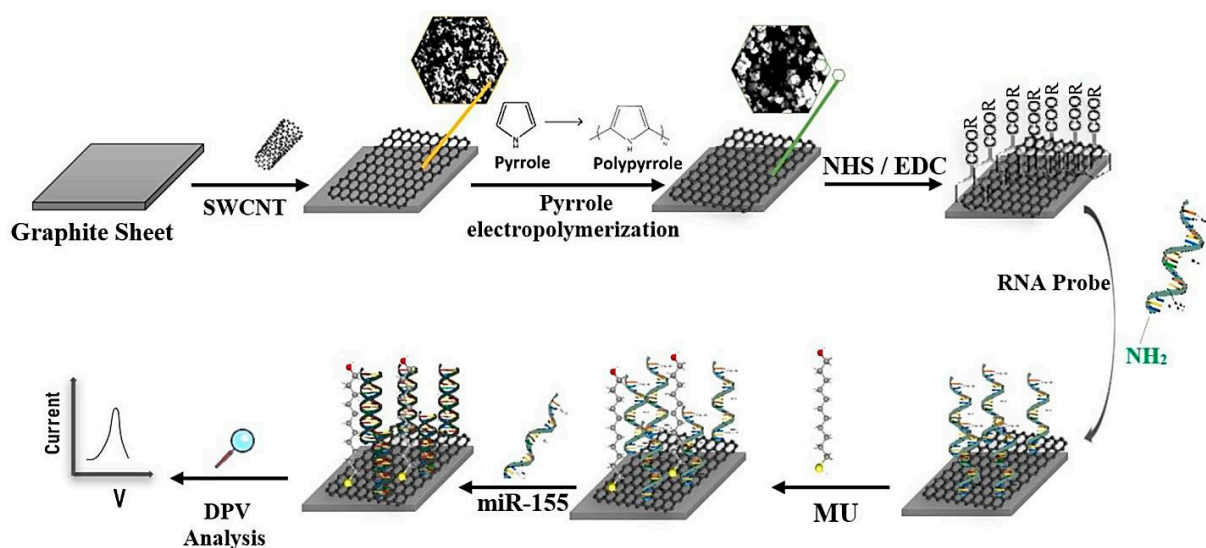
Figure 6. Schematic representation of an electrochemical aptasensor based on the SWCNTs/PPY for miR-155. Reprinted from [46], with permission.
