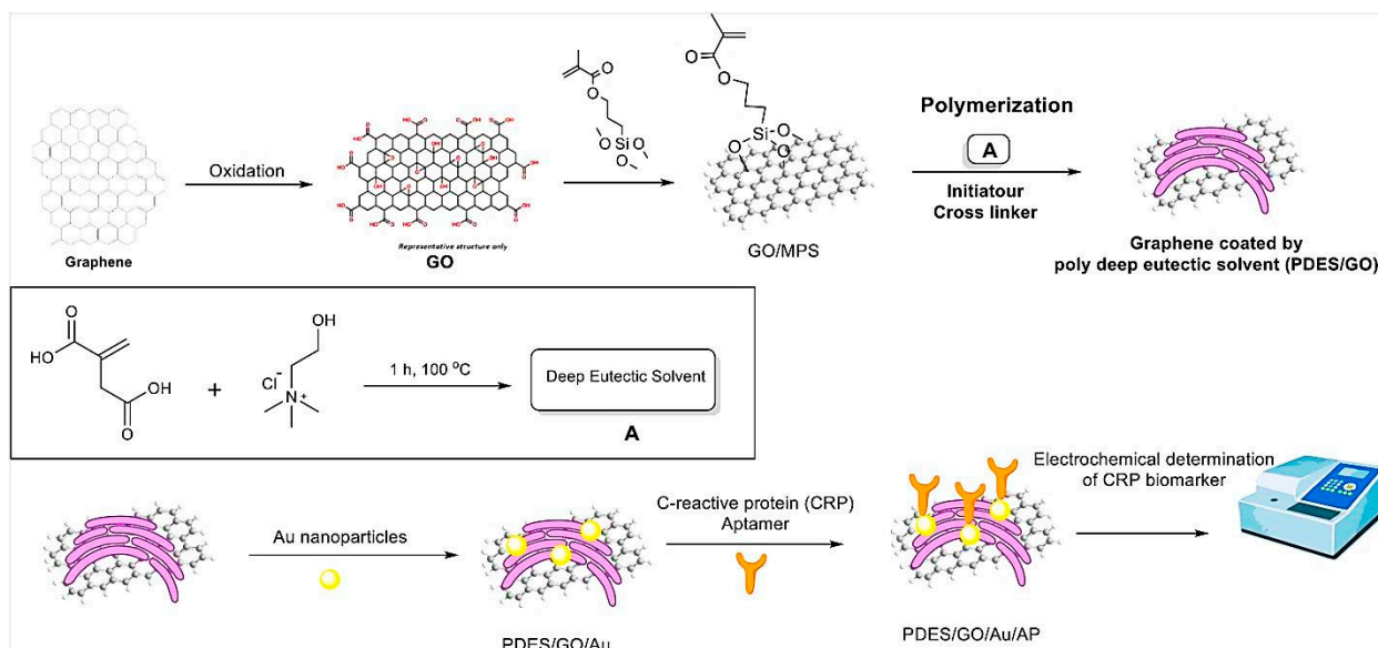
Figure 4. Schematic representation of the fabrication steps for the CRP aptasensor based on GO/PDES/AuNPs. Reprinted from Ref. [37] with permission.
