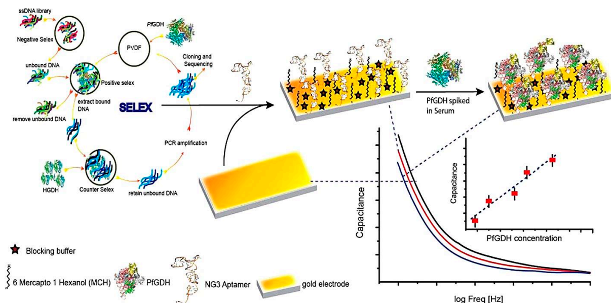
Figure 7. Schematic illustration of aptamer selection and the fabrication steps of a label-free electrochemical aptasensor for the detection of PfGDH . Reprinted from [52] with permission.
