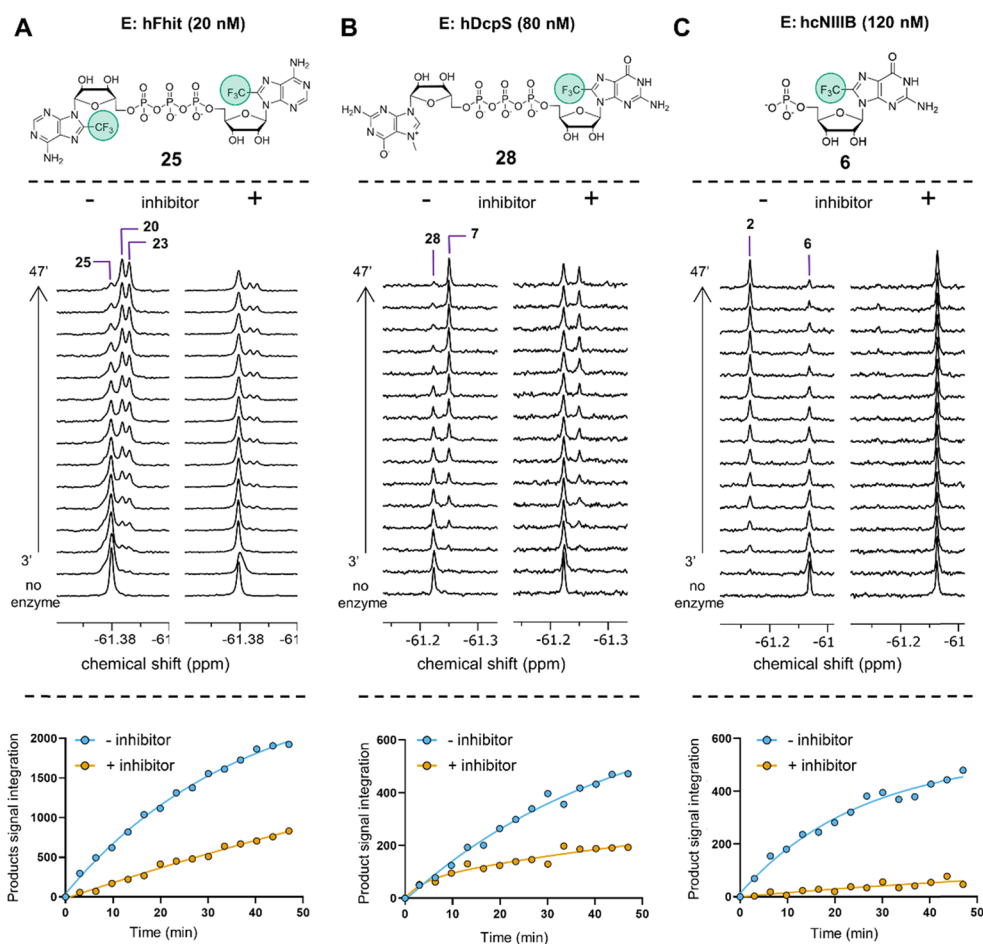
Figure 1. Monitoring enzymatic activity by ^{19}\text{F} NMR spectroscopy. (A) 25 with hFhit, (B) 28 with hDcpS, and (C) 6 with hcNIIIB. For experimental details, see the Supporting Information .
