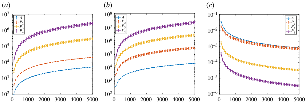
Figure 3. Evolution of average dimension, number of nonzeros and density of the non- k -cycling matrices P_k for k = 1, 2, 3, 4 corresponding to preferential attachment networks of increasing size n = 100, 200, \dots, 5000 . (a) Dimension, (b) nonzeros, and (c) density. (Online version in colour.)
