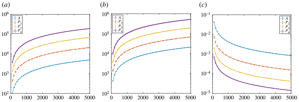
Figure 2. Evolution of average dimension, number of nonzeros and density of the non- k -cycling matrices P_k for k = 1, 2, 3, 4 corresponding to small-world networks of increasing size n = 100, 200, \dots, 5000 . (a) Dimension, (b) nonzeros, and (c) density. (Online version in colour.)
