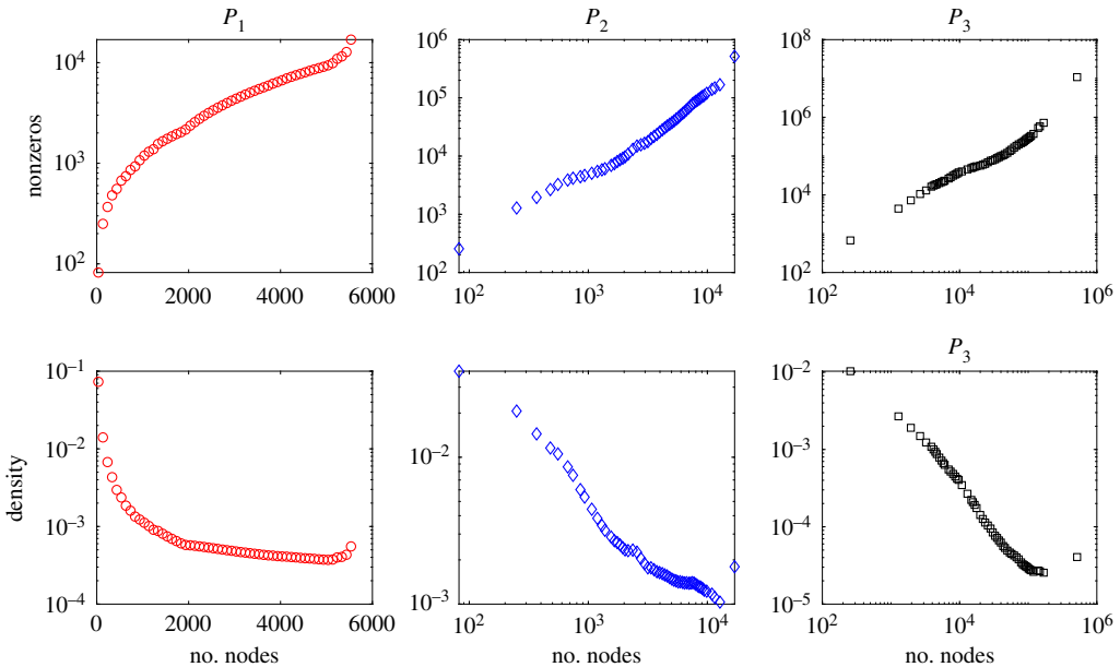
Figure 5. Evolution of number of nonzeros and of the density of the matrices P_1 = A , P_2 , and P_3 associated with subgraphs of the largest connected component of the network ERD502. (Online version in colour.)
