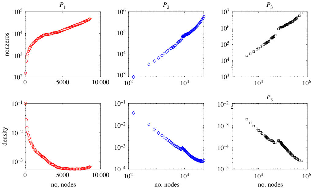
Figure 4. Evolution of number of nonzeros and of the density of the matrices P_1 = A , P_2 , and P_3 associated with subgraphs of the largest connected component of the network CA-HEP7H. (Online version in colour.)
