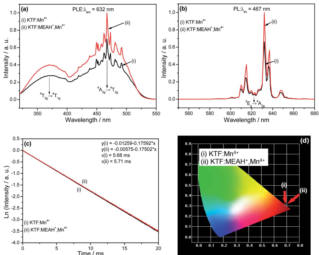
Fig. 3 Luminescent properties of two samples, (i) KTF : \text{Mn}^{4+} and (ii) KTF : \text{MEAH}^+ , \text{Mn}^{4+} : (a) and (b) PLE and PL spectra of samples (i)–(ii), (c) decay curves, (d) CIE chromaticity diagram.
