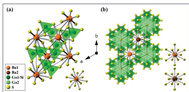
Fig. 2 (a) Schematic crystal structure of BaGa 2 Si 6 (trigonal, R\bar{3} ) and Ba 2 Ga 8 Si 16 (hexagonal, P6_3mc ) (b) viewed down the c -axis. Orange, brown, green, light green and yellow sphere balls describe Ba1, Ba2, Ga1/Si, Ga2, S and Si atoms. The insets show the coordination environment around BaS 12 (left-down) of BaGa 2 Si 6 , Ba1S 12 (right-up) and Ba2S 12 (right-down) of Ba 2 Ga 8 Si 16 .
