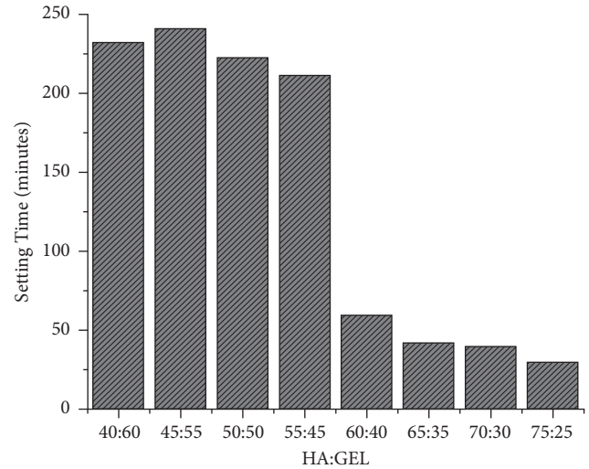
FIGURE 3: The setting time test results of IBS.
