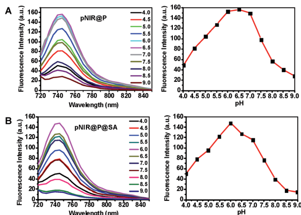
Fig. 3 pH correlated fluorescence of pNIR@P (A) and pNIR@P@SA (B). The two polymerosomes were spiked into sodium phosphate buffer (100 mM, pH 4.0–9.0) to a final concentration of 100 \mu\text{g ml}^{-1} . Fluorescence emission of the solutions was recorded using \lambda_{\text{ex}}@715 \text{ nm} and fluorescence emission intensities@745 nm were plotted over buffer pH.
