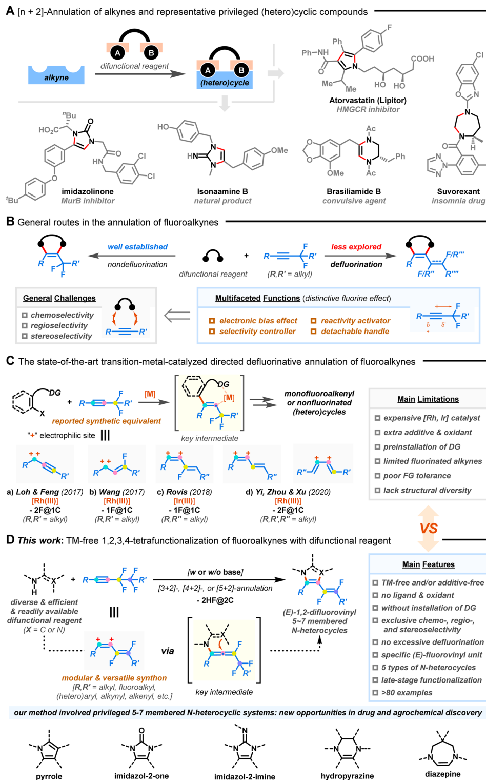
Fig. 1 Annulation of alkynes for the construction of (hetero)cyclic systems. (A) [n + 2] -annulation of alkynes and representative privileged (hetero)cyclic compounds. (B) General routes for the annulation of fluoroalkynes. (C) The state-of-the-art transition-metal-catalyzed directed defluorinative annulation of fluoroalkynes (“–2F@1C” means two C–F bond cleavages at a single carbon site; “–1F@1C” means one C–F bond cleavage at a single carbon site). (D) Divergent defluorinative [3-5 + 2] -annulation of fluoroalkynes with difunctional reagents (this work).
