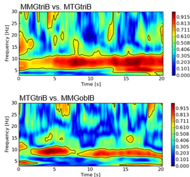
Figure 4. Exemphary wavelet coherence spectra (intrapersonally). The diagrams show the wavelet coherence spectra of the intrapersonal signal pairs of triceps muscle vs. its tendon (above) and of the triceps tendon vs. the abdominal external oblique muscle (bottom) of subject B during isometric interaction of subject A and B at 80% of the MVC.
