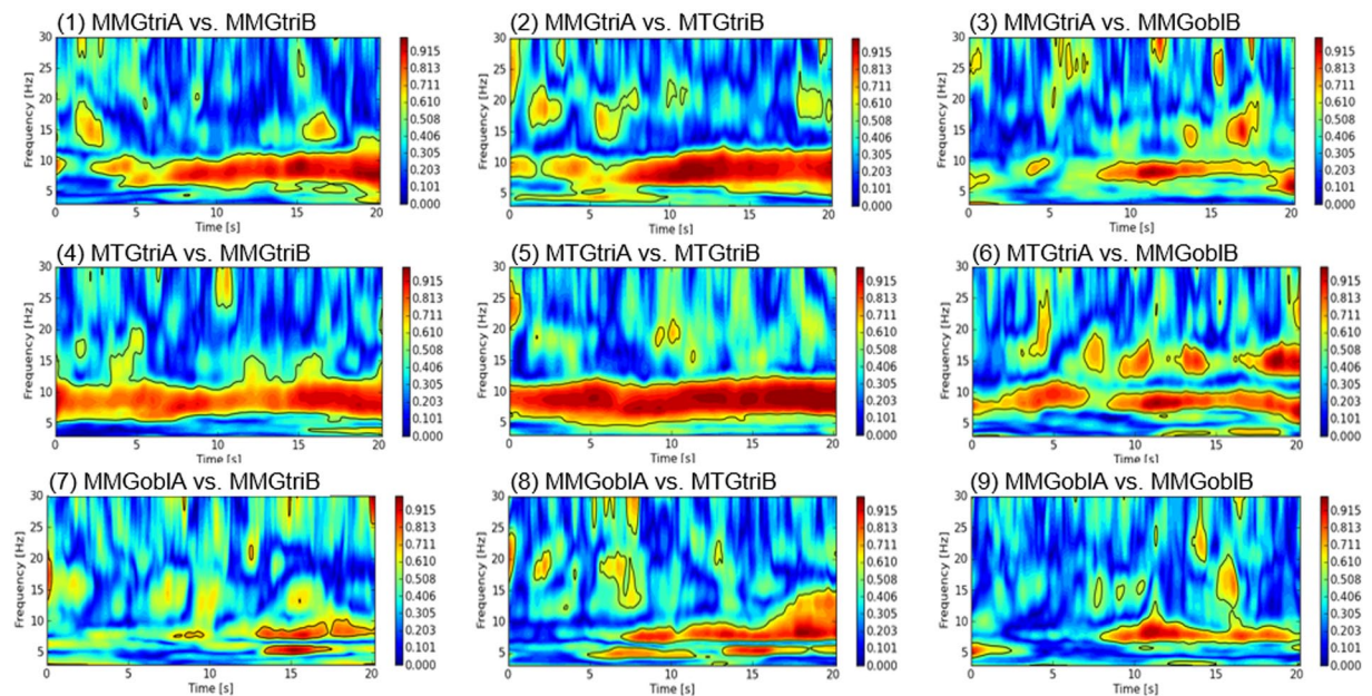
Figure 3. Exemphary wavelet coherence spectra (interpersonally). The diagrams show the wavelet coherence spectra of all three MMG- and MTG-signals of one pair (subject A and B) during one trial of isometric interaction at 80% of the MVC. The intensity of coherence (right scale) in the frequency range of 3 to 30 Hz (y-axis) over the time in s (x-axis) is displayed. The black bordered areas show pointwise significant areas of coherence.
