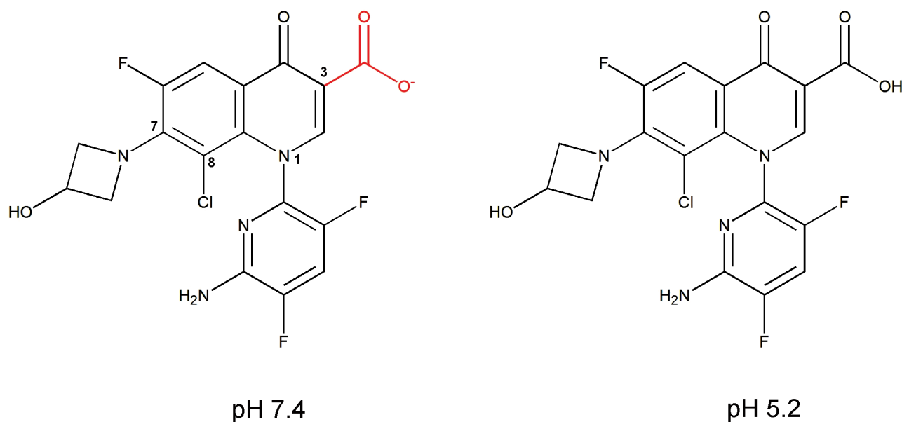
Figure 1. Chemical structure of delafloxacin with atom numbering for the key positions discussed in the text. Due to the lack of basic group in the C7 substituent, the only ionizable group is the carboxylate function attached to position C3 (calculated pK_a = 5.43 ). The figure shows the calculated predominant forms at pH 7.4 (left; anionic [to 98.5%]) and at pH 5.2 (right; neutral [62.7%]). Calculations were made with MarvinSketch version 18.9.0 (academic license) available from http://www.chemaxon.com .
