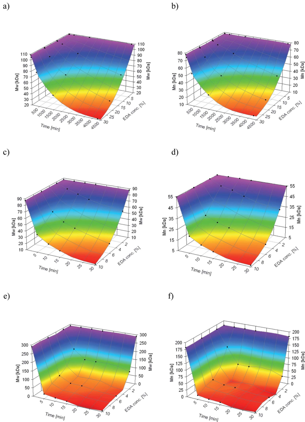
Fig. 6 Change of \overline{M}_w of (a) PCL, (c) PLCL, and (e) PLLA, and \overline{M}_n of (b) PCL, (d) PLCL, and (f) PLLA vs. EDA concentration and reaction time.
