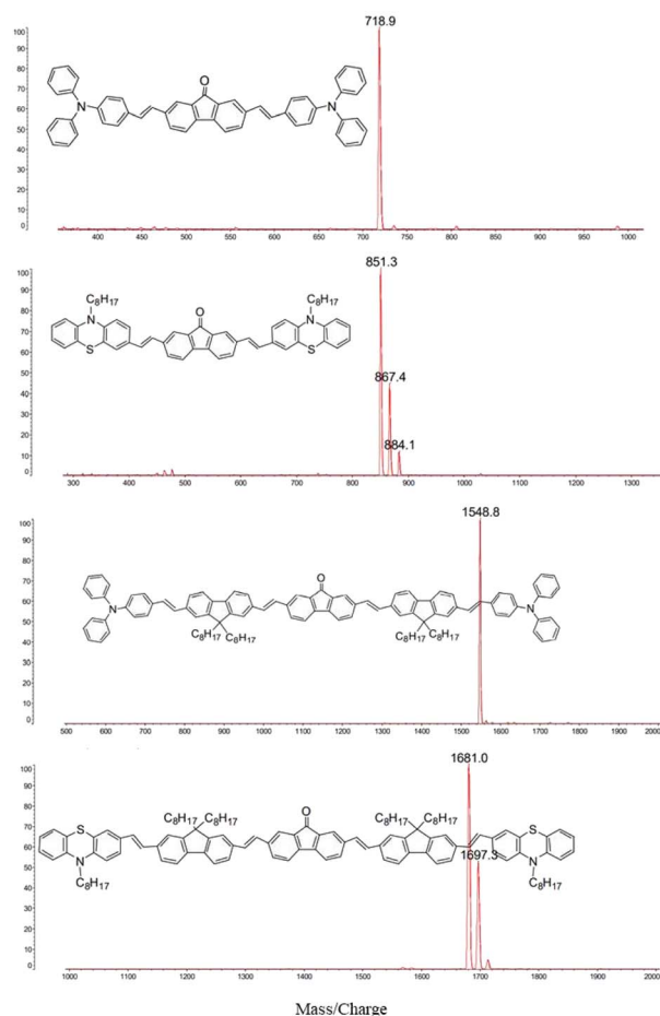
Fig. 1 The MALDI/TOF MS spectra of compound #1–#4 with 1,8,9-trihydroxyanthracene as a matrix.
