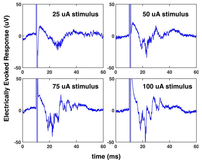
Figure 2. Representative EER traces in the visual cortex of a normal rat for increasing stimulus current amplitude delivered to the retina. Each trace is averaged over 50 trials. Stimulus pulse is delivered at 10 ms for each stimulus amplitude.
