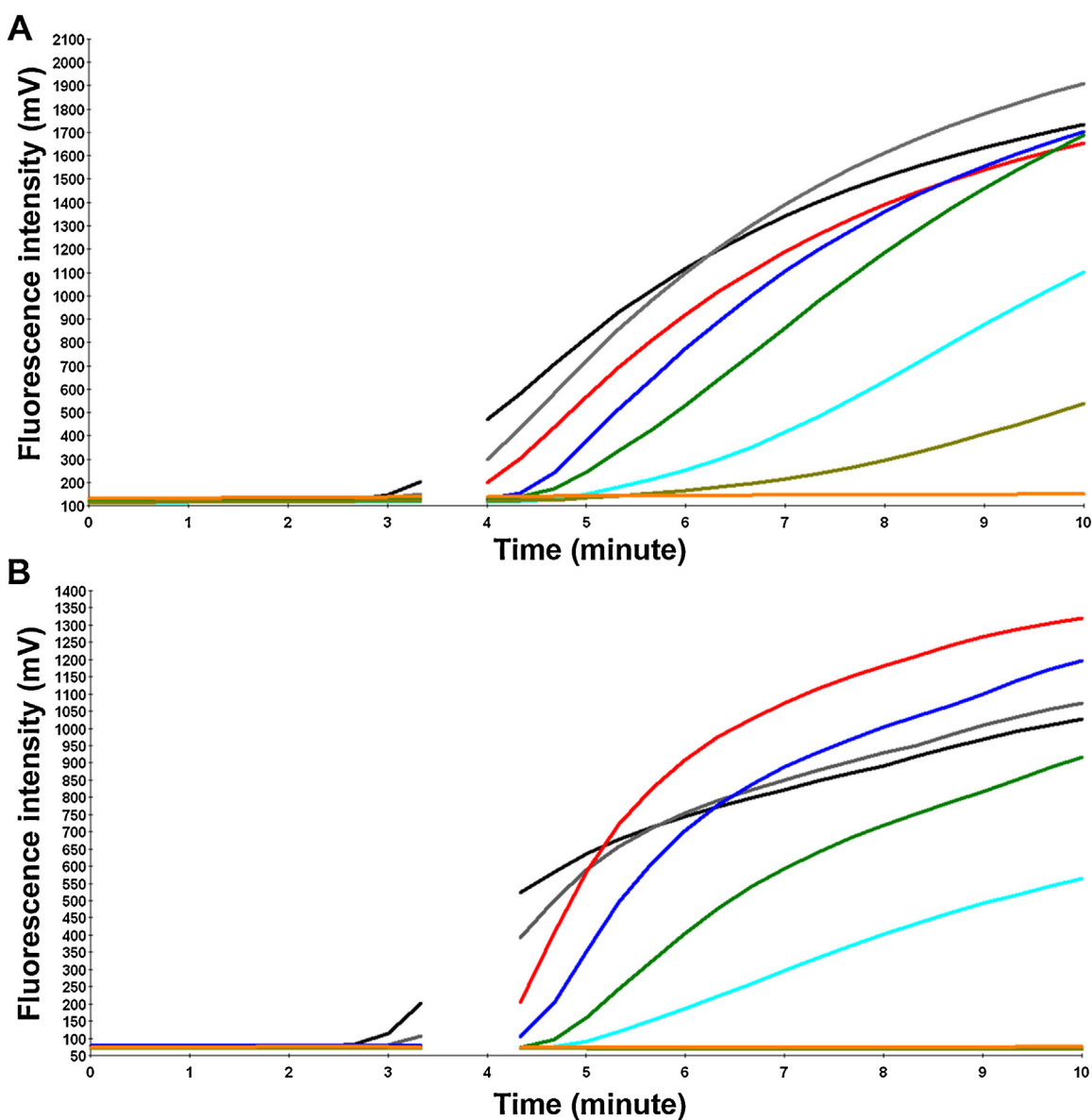
Fig. 3. Analytical sensitivity of H7N9 RT-RPA assays. (A) The H7 and (B) the N9 RT-RPA assays. Fluorescence development via real-time detection using a dilution range of 10^7 – 10^1 RNA molecules/ \mu l of the H7 and N9 RNA molecular standards (graph generated by ESEquant tube scanner studio software). The sensitivities were 10 and 100 RNA molecules for the H7 (A) and the N9 (B) RT-RPA assays, respectively. The reverse transcription took place in the first minute. To increase the sensitivity, a mixing step was performed after 3 min (no fluorescence signal was detected). 10^7 represented by black line; 10^6 , gray; 10^5 , red; 10^4 , blue; 10^3 , green; 10^2 , cyan; 10^1 , dark khaki; and negative control, orange. (For interpretation of the references to color in this text, the reader is referred to the web version of the article.)
