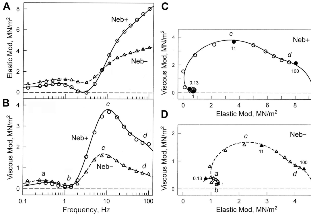
Figure 3. Comparison of complex moduli of Neb + and Neb - fibers. (A and B) Elastic modulus (Mod; A), and viscous modulus (B), plotted as functions of frequency. (C and D) The same data are plotted in Nyquist plots. In B–D, a, b, c, and d indicate characteristic frequencies, identifying individual exponential processes. These are defined in Eq. 1 and represent the speed (kinetics) of force transients. Discrete points represent the measured data, and curves represent best fits to Eq. 1. The unit of moduli is MN/m 2 = MPa, where M = mega = 10 6 , N = Newton, and Pa = Pascal.
