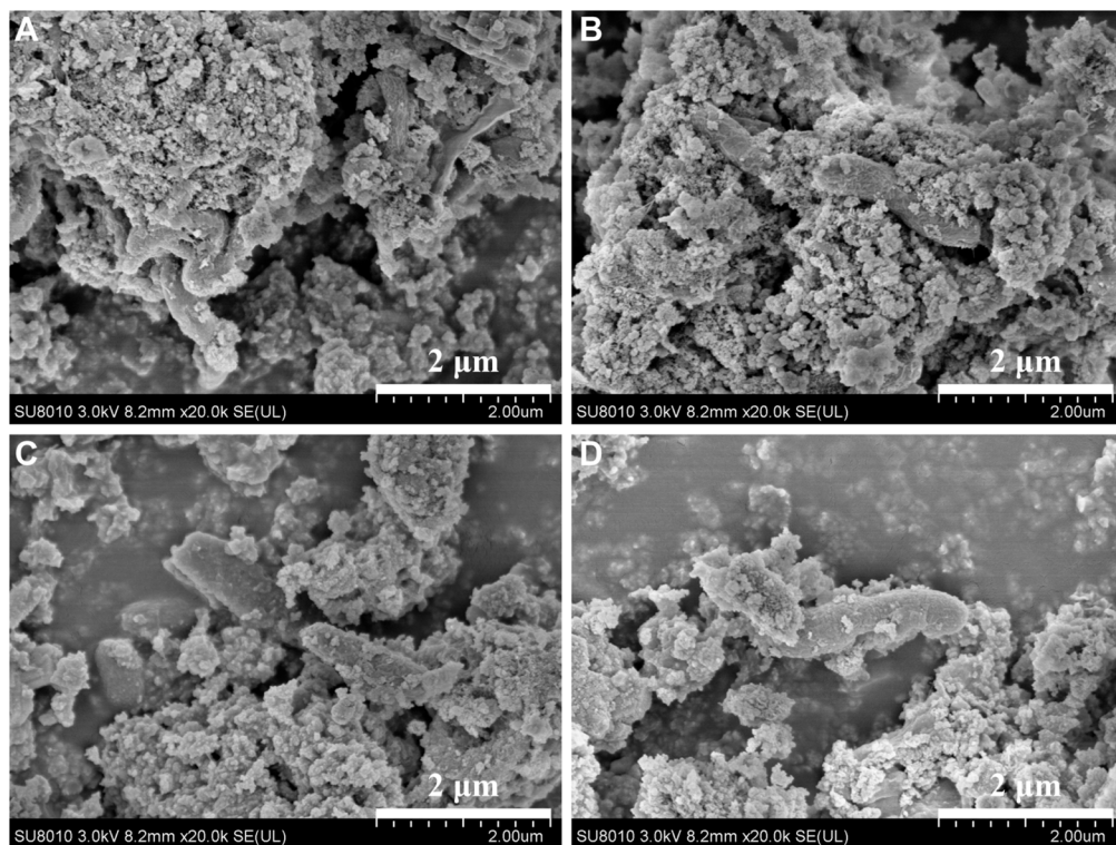
Fig. 3 The microscopic morphology of different microorganisms in the activated sludge samples taken from the biological reaction tanks of A1 (A), O1 (B), A2 (C), and O2 (D) in the full-scale two-stage A/O coking wastewater treatment process.
