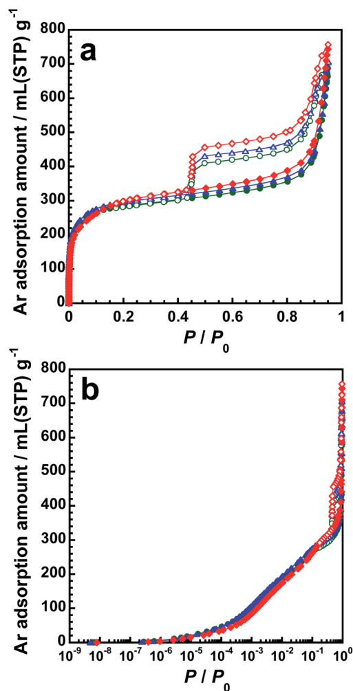
Fig. 6 Adsorption–desorption isotherms of Ar at 87 K in (a) linear and (b) logarithmic scales on p-BN-1473 (green), p-BN-1573 (blue) and p-BN-1673 (red).
