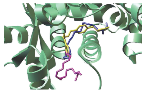
FIGURE 3: Representative binding mode of the most stable docked orientation of catalpic acid and punicalic acid with peroxisome proliferator-activated receptor \gamma (PPAR \gamma ). The PPAR \gamma model is shown in ribbon mode. Catalpic acid and punicalic acid poses generated by AutoDock Vina are colored in blue and magenta, respectively. Rosiglitazone is colored in yellow.
