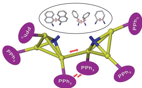
Scheme 1 Possible intramolecular interaction and conformational change in diamino-centered chiral Au 6 clusters.
