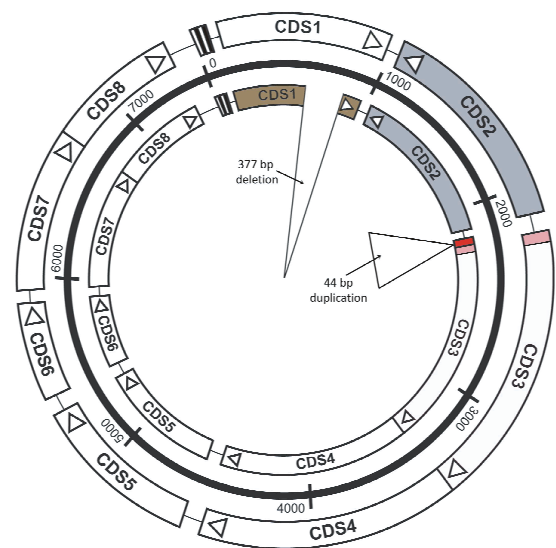
Figure 3 Comparison of plasmids pSW2 (inner circle) and pSW3 (outer circle). pSW2 carries a 377 bp deletion in CDS1 (coloured brown for pseudogene) and a 44 bp duplication immediately upstream of CDS3 (shown in red). CDS2 is transcribed in the opposite direction to the other CDSs and is shaded grey. The set of 22 bp repeats upstream of CDS1 form the putative origin of replication.
