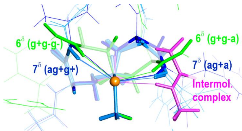
Figure 6. Comparison of the \text{NH} \cdots \text{Se} approaches of the relevant conformations ( 5\text{-}7_{g+/g-}^{\delta} light blue, 5\text{-}7^{\delta}/5_a\text{-}\pi dark blue and 6^{\delta}\text{-}\pi_{g+}\text{-}10 green) of the Ac-Sem-Phe- \text{NH}_2 compound, as found at the DFT-D level of theory. The terminal part of all the Sem side-chains was overlaid (Se atom in dark yellow), allowing to distinguish the effect of the \chi_3 dihedral orientation (side-chain dihedrals between parentheses). For the sake of clarity, front atoms were omitted and background atoms shaded. For reference, the structure of the \text{MAA} \cdots \text{S-SeMe}_2 intermolecular complex was also added. The same figure for the Ac-Met-Phe- \text{NH}_2 compound, provided as Figure S1 in the Supplementary Material, illustrates the similarities between the two species.
