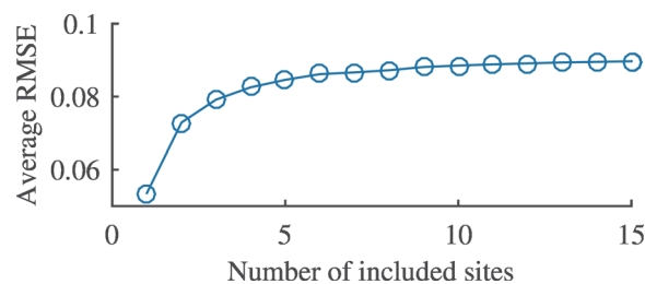
Fig 4. Influence of the number of included sites in the model development. Average root mean squared error (RMSE) of the model with respect to the number of included sites. Statistics are based on developing the model 1000 times for each included sites size.
