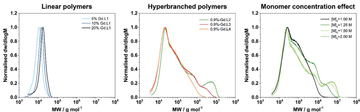
Fig. 3 SEC molecular weight (MW) distribution of selected linear and hyperbranched copolymers demonstrating: (left) low \mathcal{D} of linear copolymers and increasing MW as the ratio of Gd·L 1 : NAM increases; (centre) high MW shoulder and broad distribution of MW when a crosslinker is introduced; (right) increase in high MW content as initial concentration of monomer is increased.
