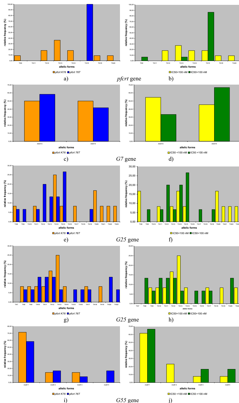
Figure 1 Microsatellite allelic frequencies of pfcr1 and putative transporter genes in 27 P. falciparum isolates according to pfcr1 K76 allele and chloroquine response phenotype. Microsatellite allelic relative frequencies are given according to pfcr1 K76 (wild allele, orange bars) or pfcr1 K76T (mutant allele, blue bars) (Figure a, c, e, g and i), or according to inhibitory concentration values (IC 50 ) for chloroquine (susceptible isolates, yellow bars; resistant isolates, green bars) (Figure b, d, f, h and j). The relative frequency of the various allelic forms within each haplotype subgroup is indicated. The microsatellites have either (AAAT) n alleles or (TA) n alleles and they are classified according to the number ( n ) of repeats. Figure a, b: pfcr1 microsatellite in intron 4; Figure c, d: G7 microsatellite; Figure e, f: G25 microsatellite in intron 3; Figure g, h: G25 microsatellite in intron 4; and Figure i, j: G55 microsatellite. Motif 1: TAATATTATAATAT(TA) 9 T Motif 2: TAATAT(TA)IIT Motif 3: TAATAT(TA)I0T Motif 4: TAATAT(TA) 9 T.
